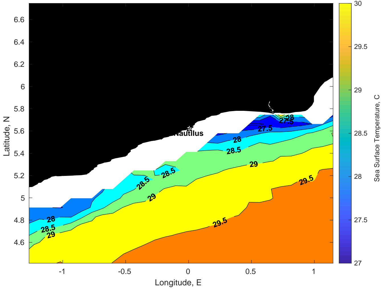
SST for Nautilus at 28-Mar-2025 00:00:00
