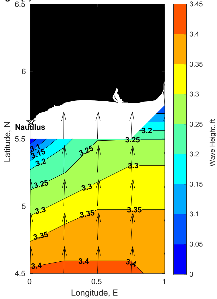
Wave Height (ft) for Nautilus at 29-Mar-2025 09:00:00
