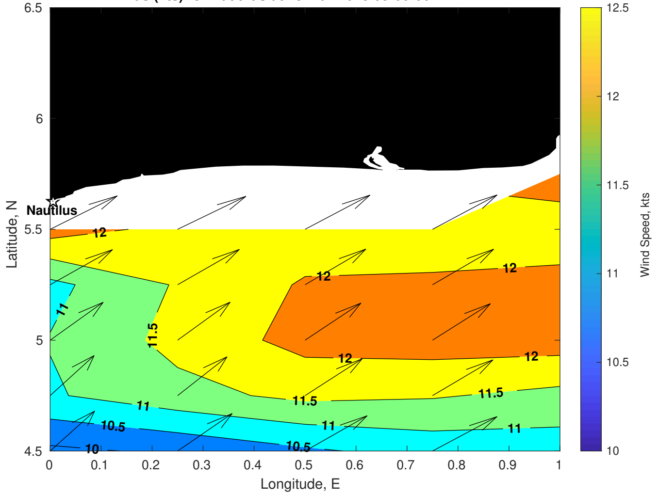
Winds (kts) for Nautilus at 29-Mar-2025 09:00:00
