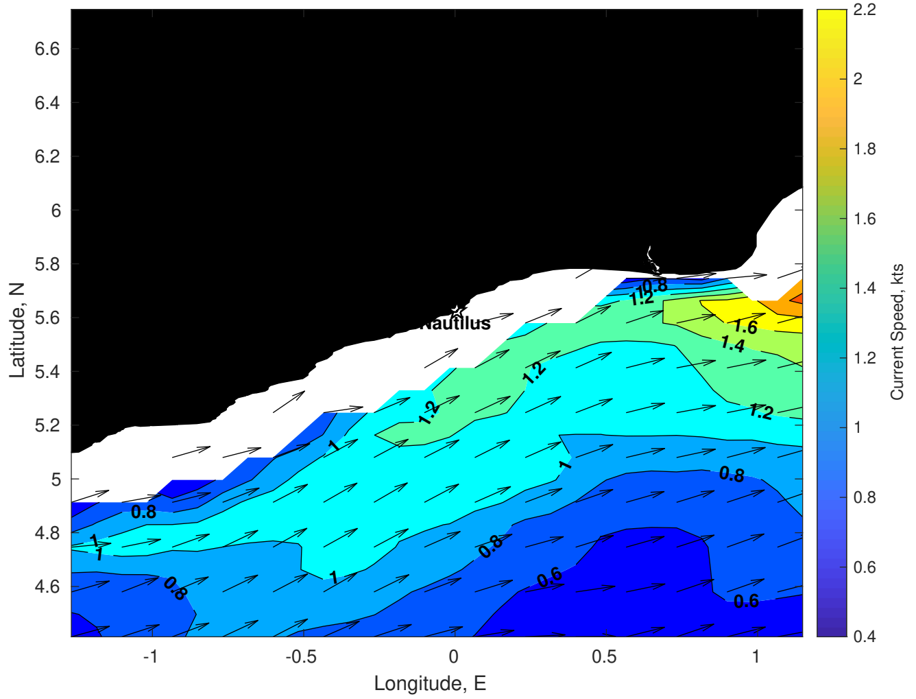
Surface Currents for Nautilus at 28-Mar-2025 00:00:00
