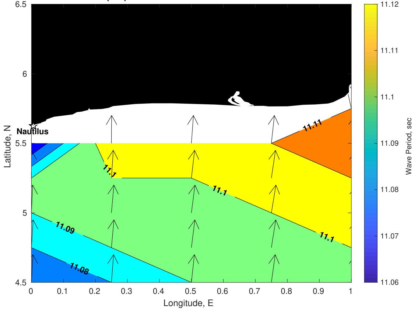
Wave Period (sec) for Nautilus at 29-Mar-2025 09:00:00
