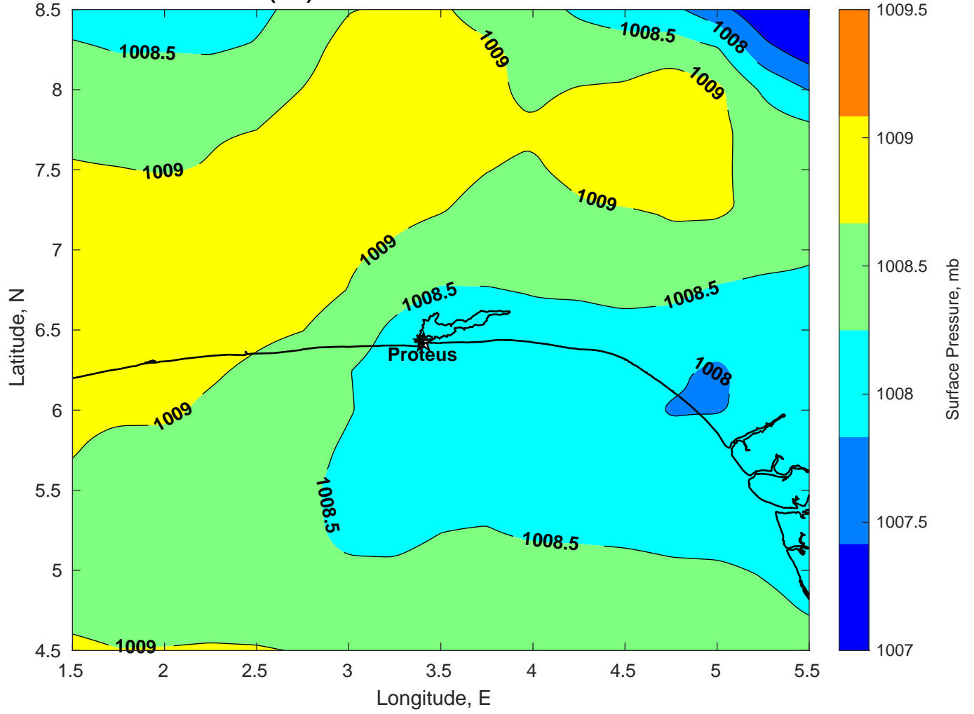
Surface Pressure (mb) for Proteus at 29-Mar-2025 00:00:00
