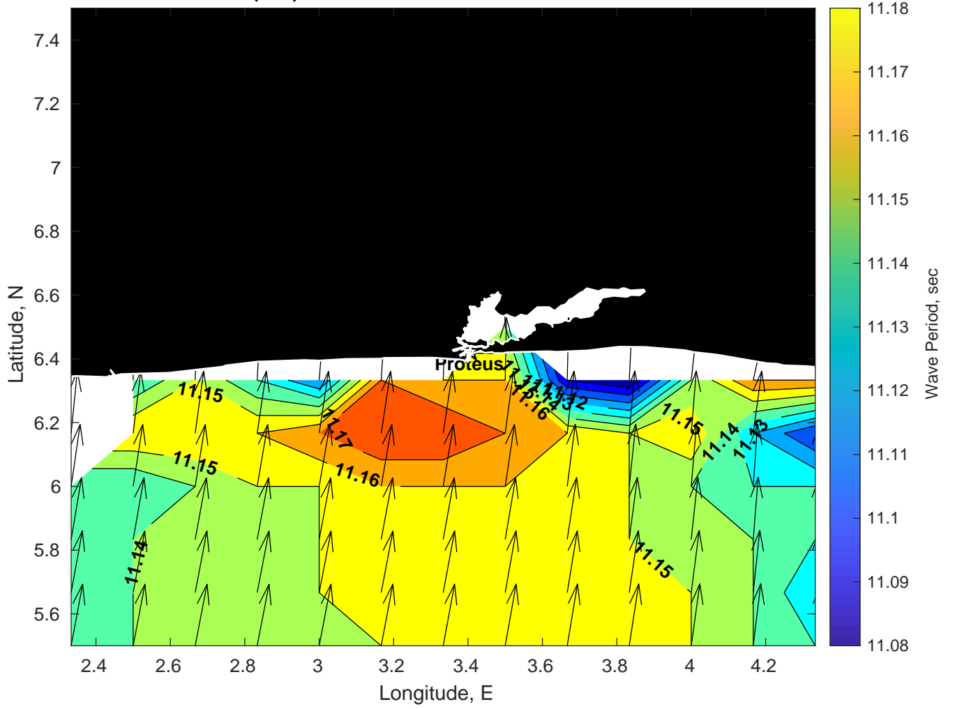
Wave Period (sec) for Proteus at 29-Mar-2025 09:00:00
