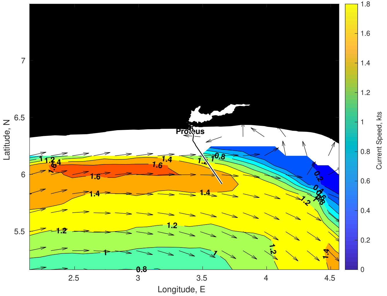
Surface Currents for Proteus at 28-Mar-2025 00:00:00
