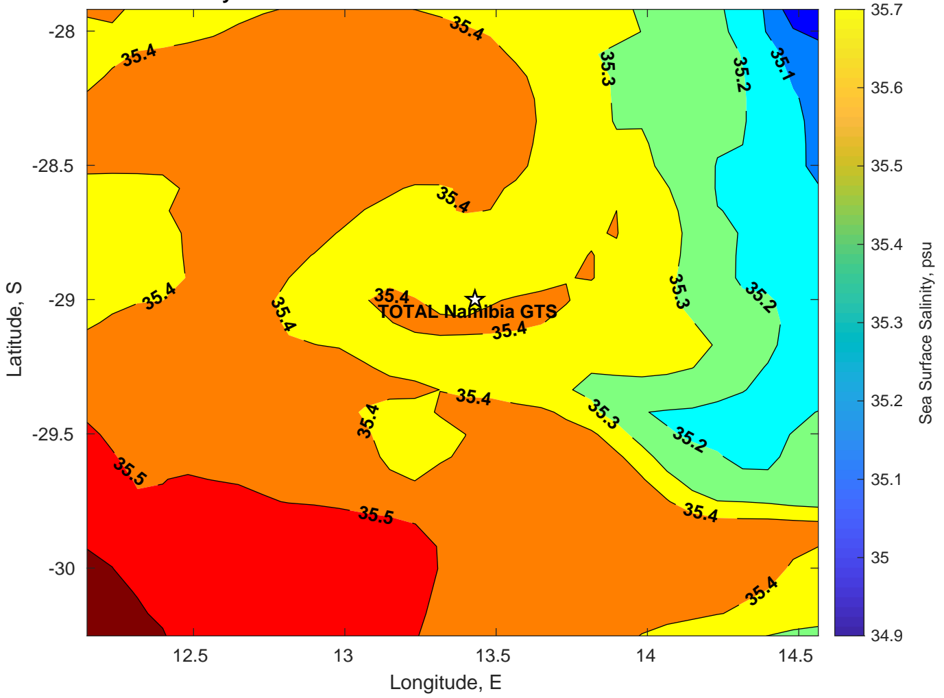
Surface Salinity for TOTAL Namibia GTS at 28-Mar-2025 00:00:00
