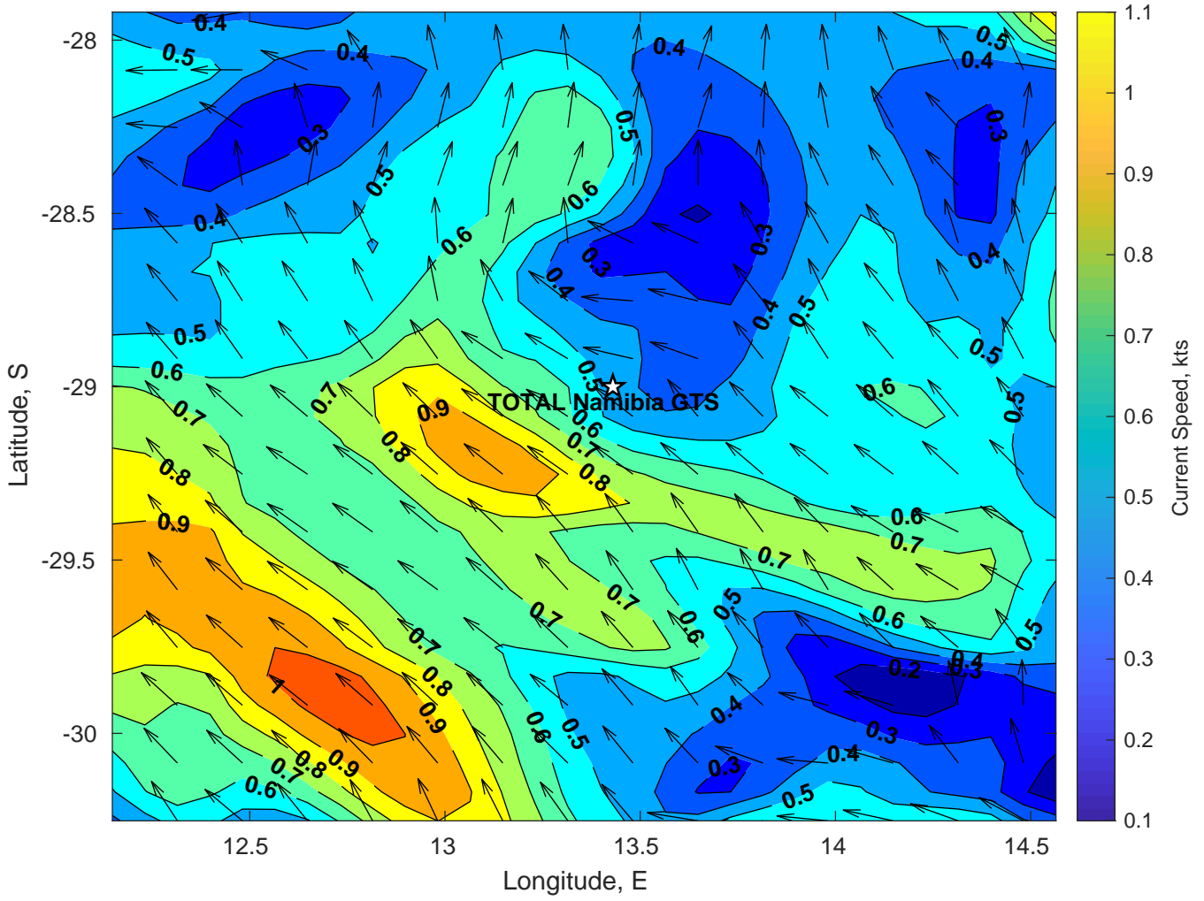
Surface Currents for TOTAL Namibia GTS at 28-Mar-2025 00:00:00
