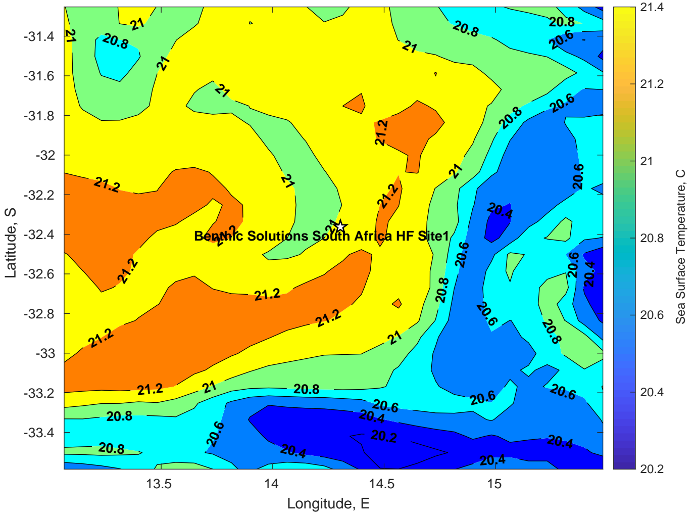
SST for Benthic Solutions South Africa HF Site1 at 29-Mar-2025 00:00:00
