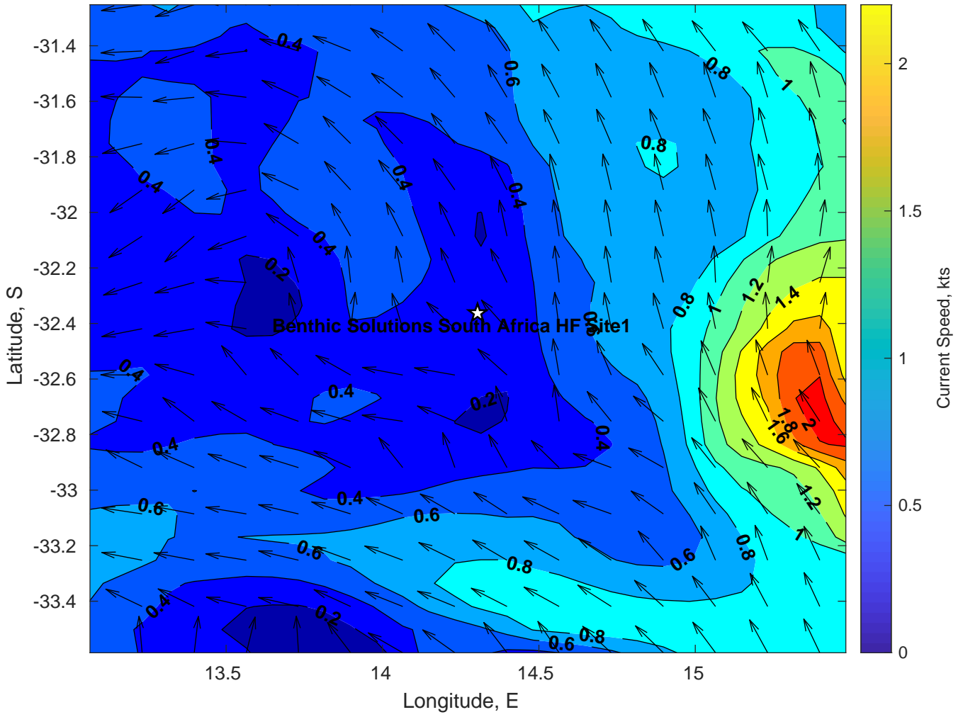
Surface Currents for Benthic Solutions South Africa HF Site1 at 29-Mar-2025 00:00:00
