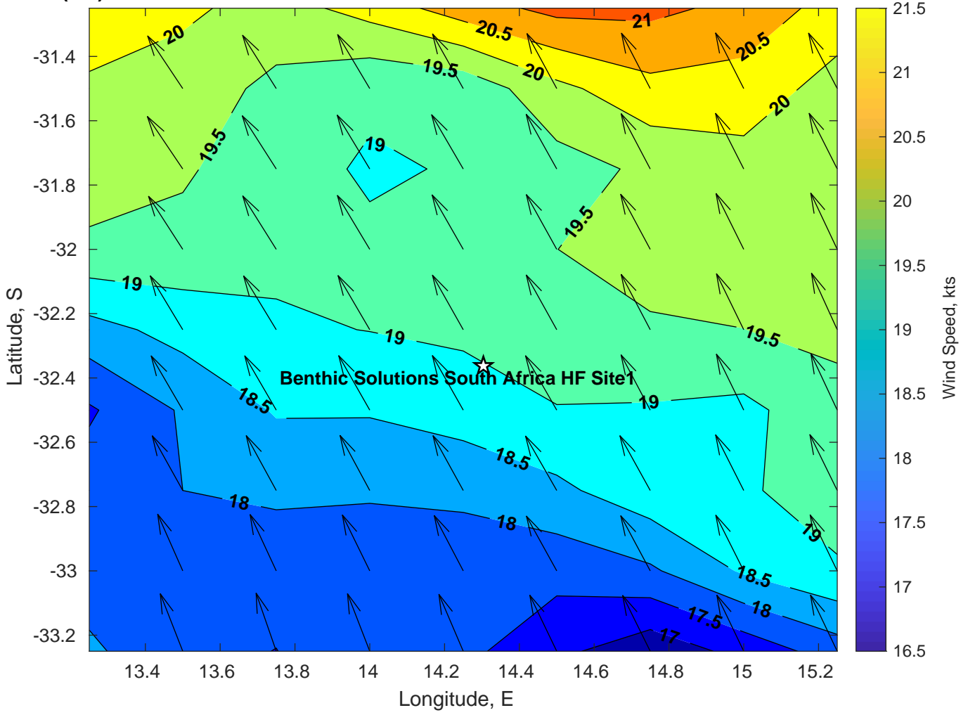
Winds (kts) for Benthic Solutions South Africa HF Site1 at 30-Mar-2025 09:00:00
