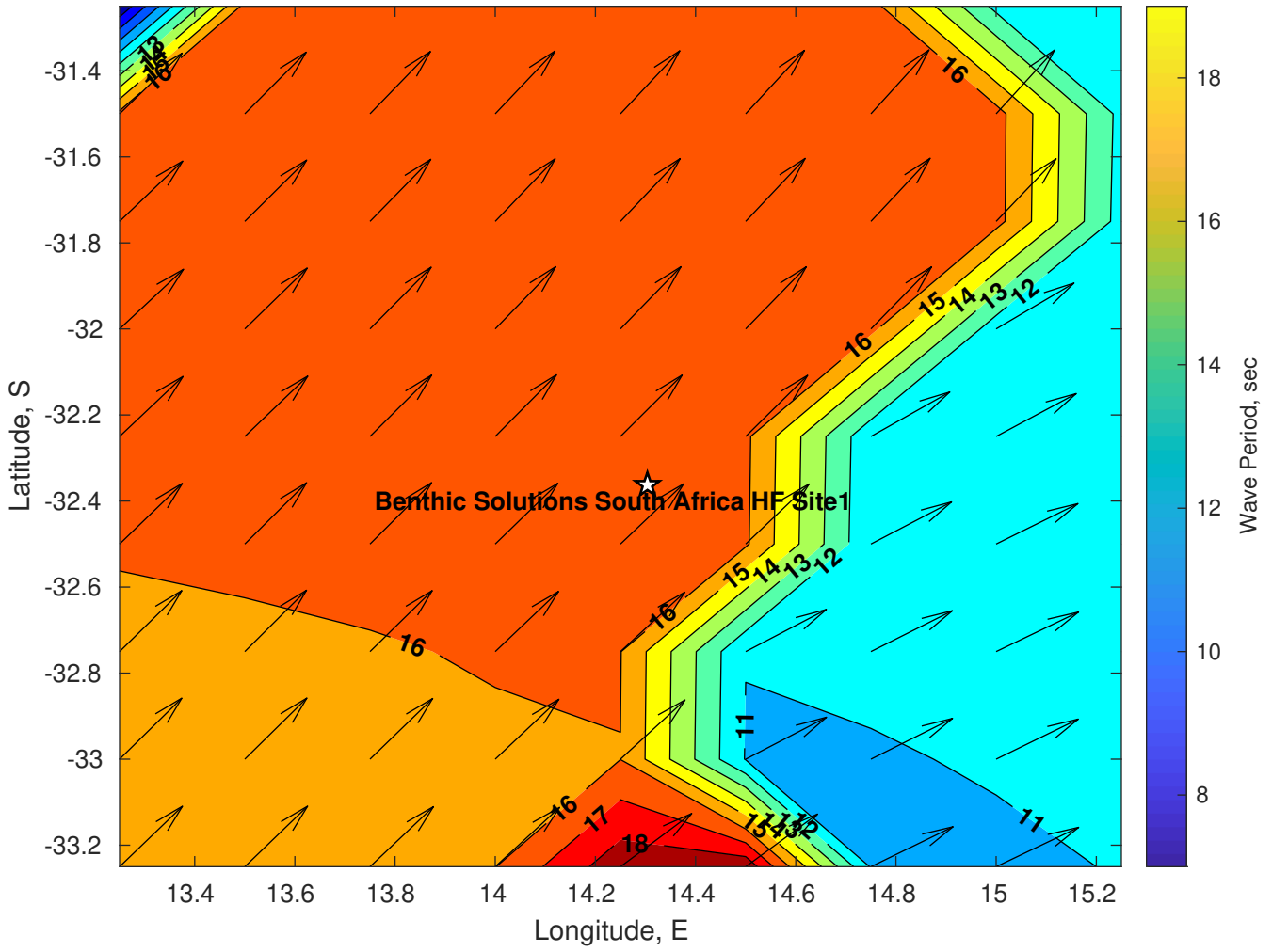
Wave Period (sec) for Benthic Solutions South Africa HF Site1 at 30-Mar-2025 09:00:00
