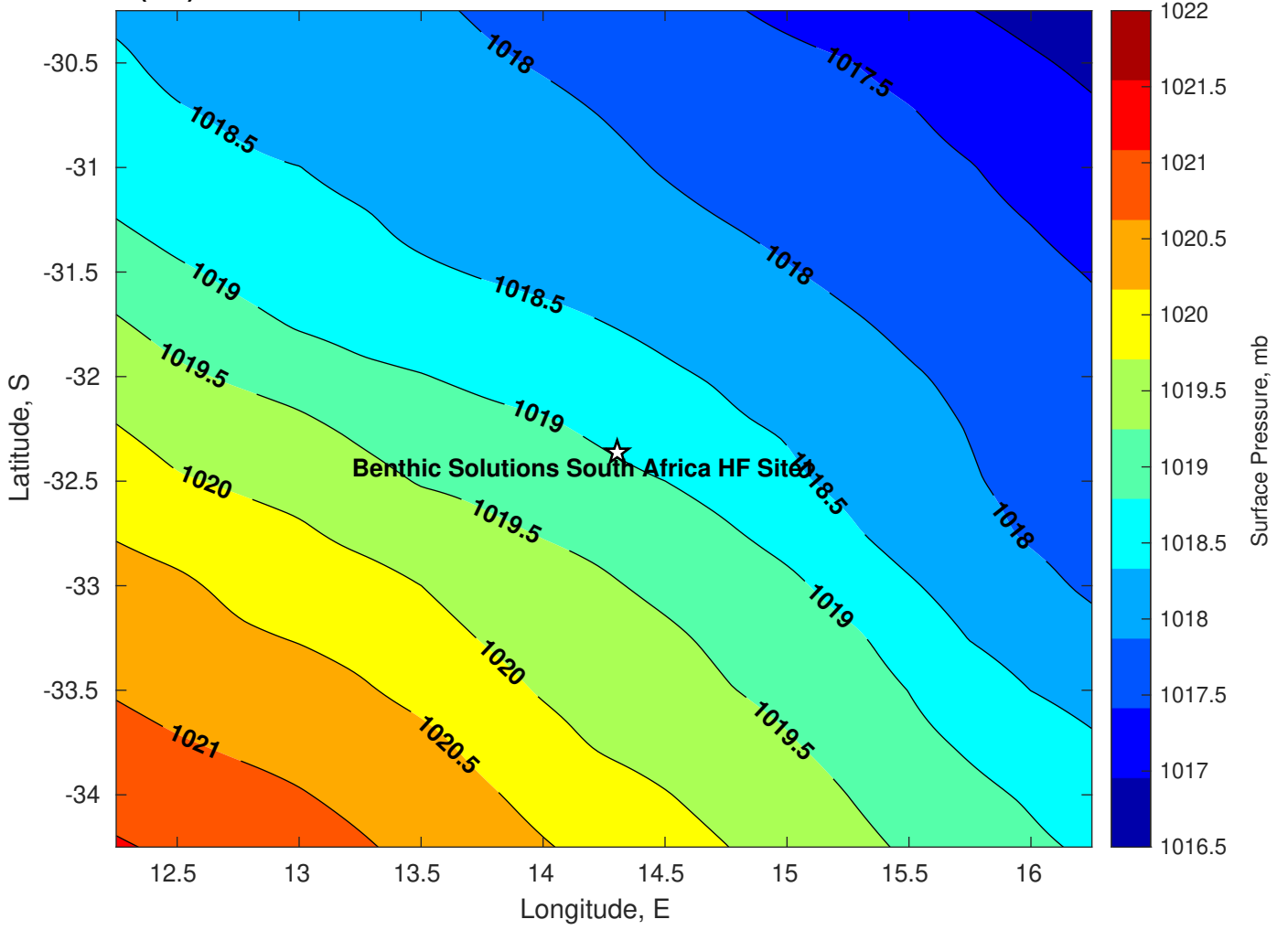
Surface Pressure (mb) for Benthic Solutions South Africa HF Site1 at 30-Mar-2025 00:00:00
