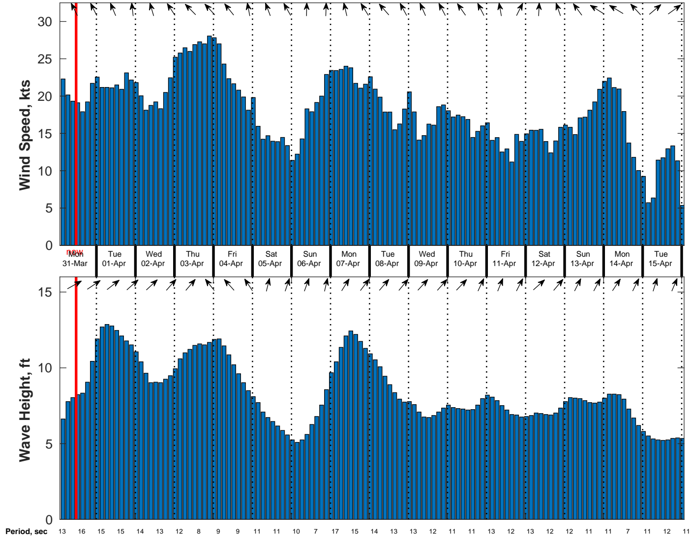
Wind & Wave Forecast for Benthic Solutions South Africa HF Site1 from 30-Mar-2025 02:00:00 to 15-Apr-2025 02:00:00
