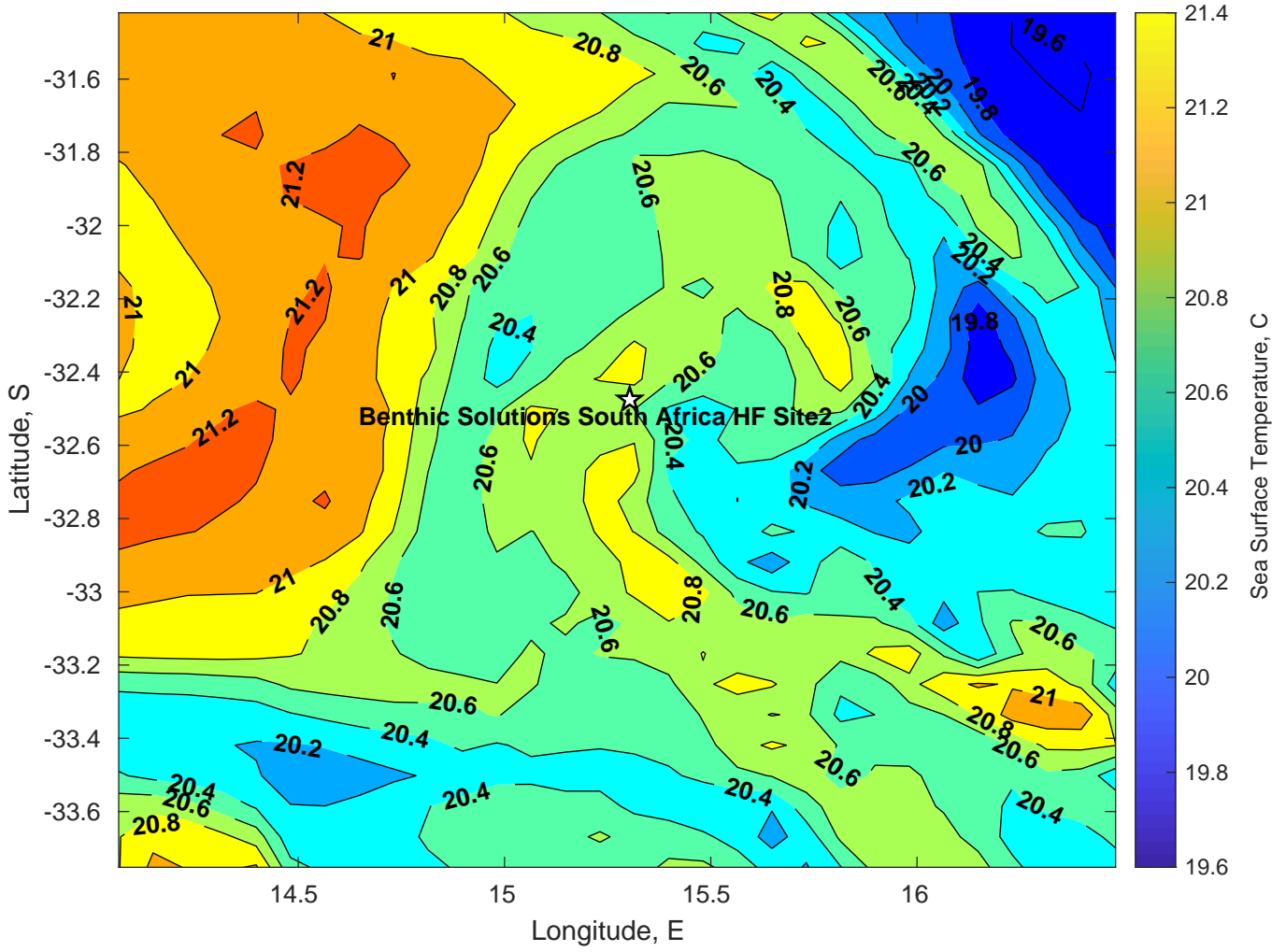
SST for Benthic Solutions South Africa HF Site2 at 29-Mar-2025 00:00:00
