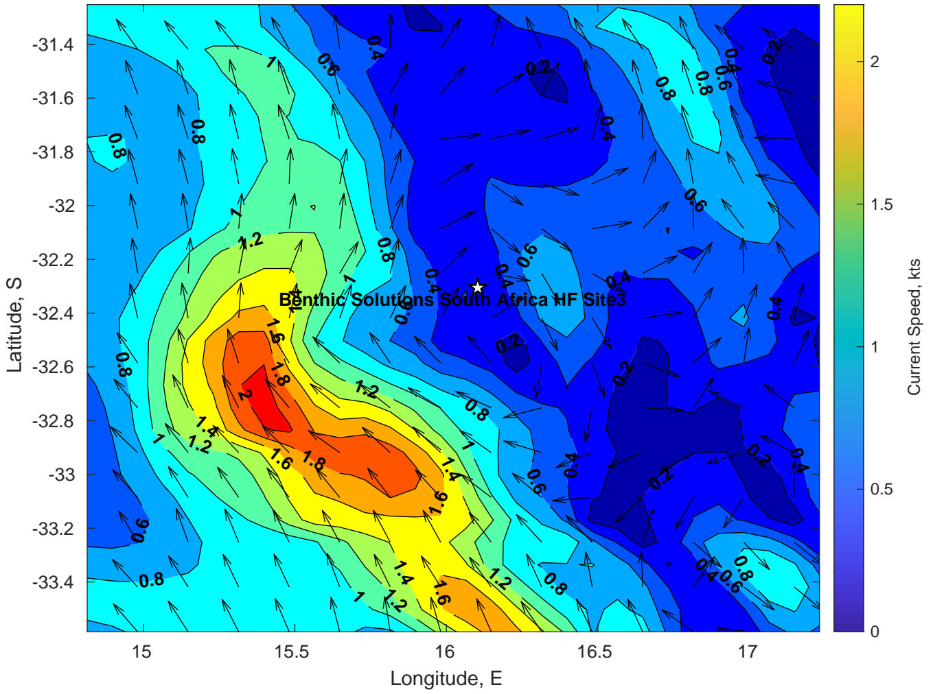
Surface Currents for Benthic Solutions South Africa HF Site3 at 29-Mar-2025 00:00:00
