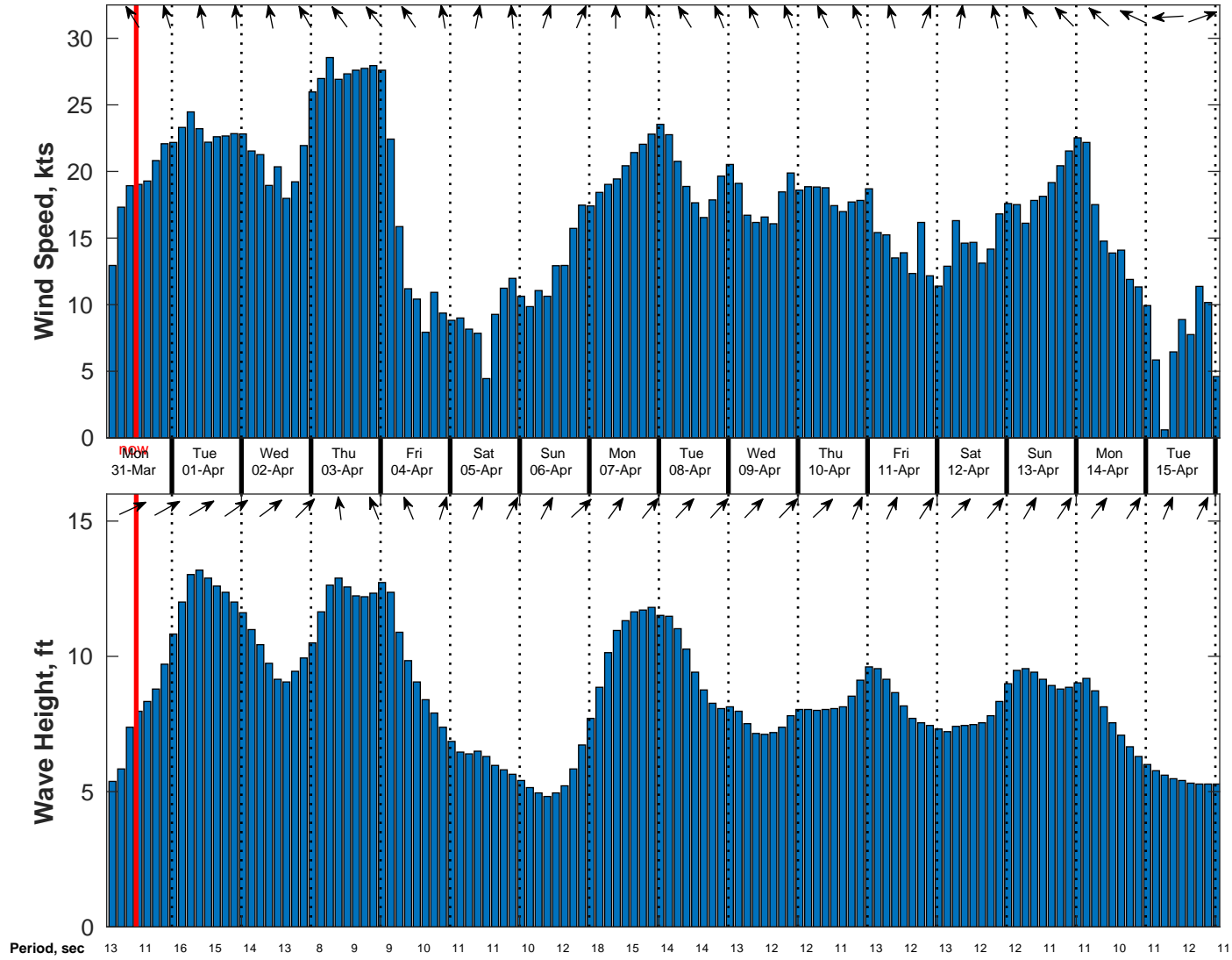
Wind & Wave Forecast for Benthic Solutions South Africa HF Site3 from 30-Mar-2025 02:00:00 to 15-Apr-2025 02:00:00
