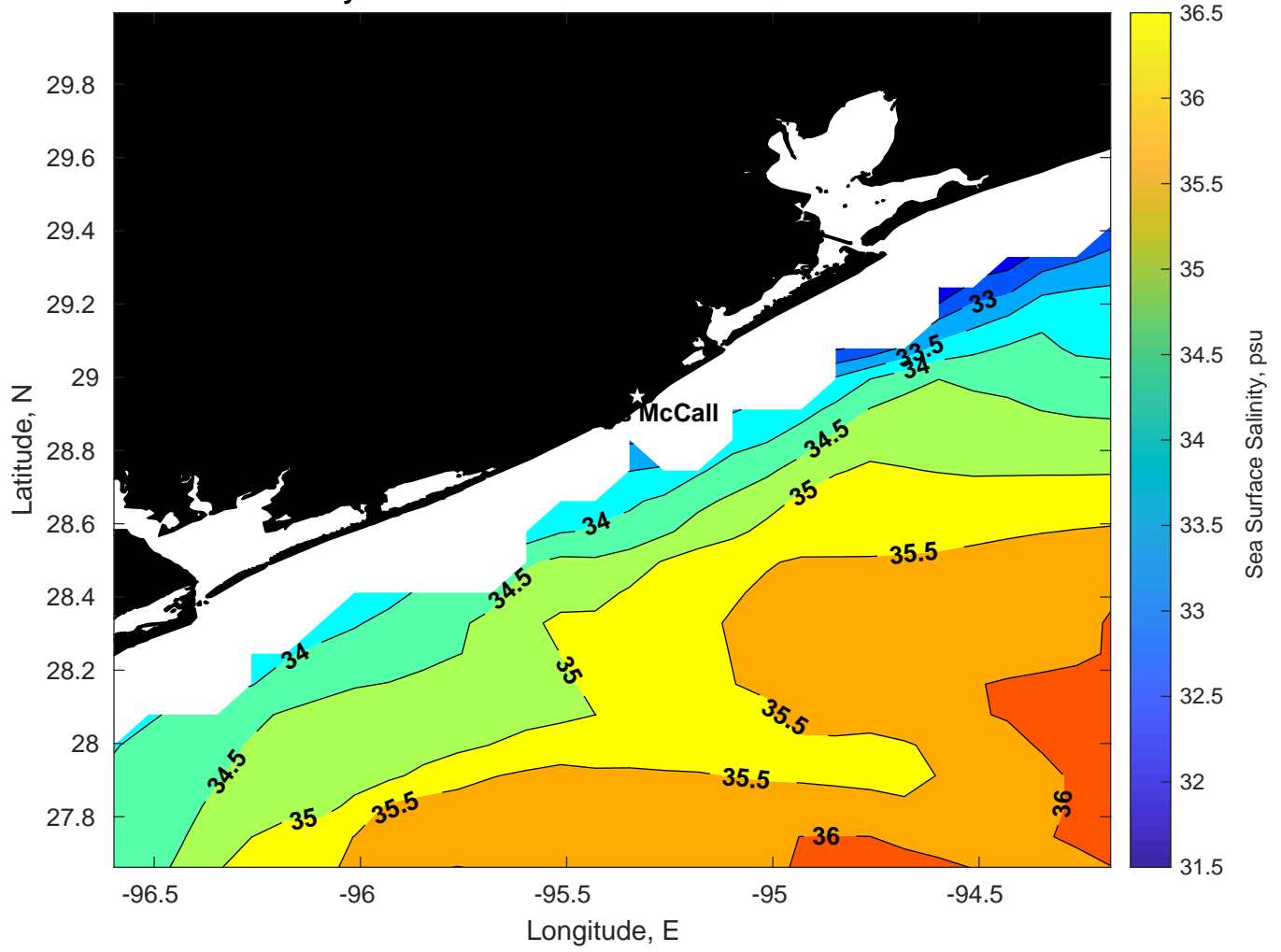
Surface Salinity for Brooks McCall at 29-Mar-2025 00:00:00
