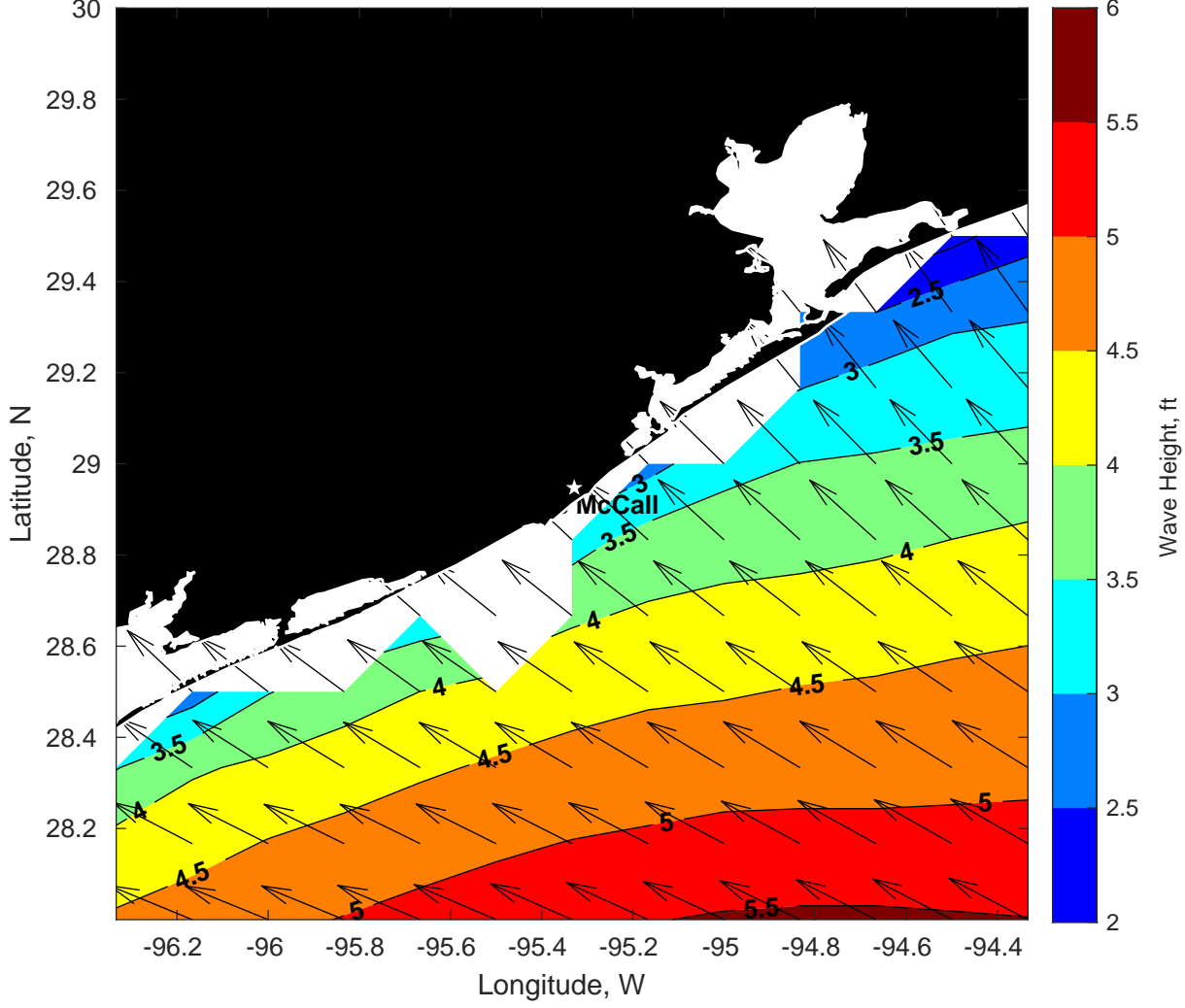
Wave Height (ft) for Brooks McCall at 30-Mar-2025 09:00:00
