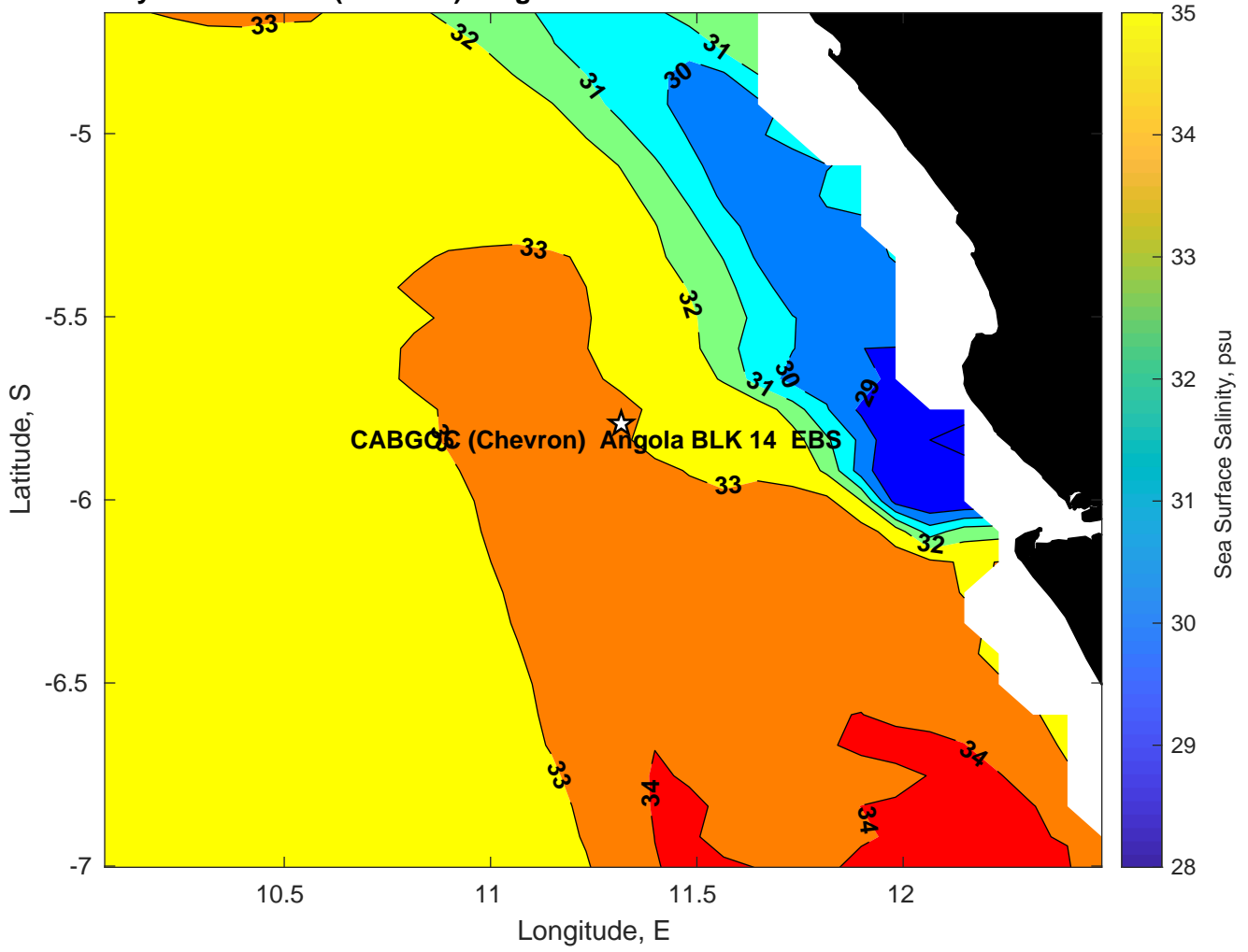
Surface Salinity for CABGOC (Chevron) Angola BLK 14 EBS at 29-Mar-2025 00:00:00
