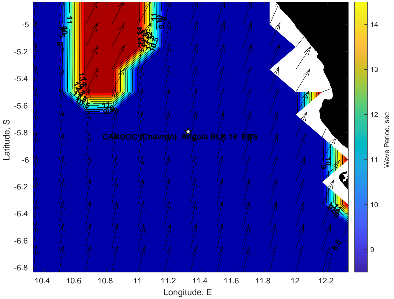
Wave Period (sec) for CABGOC (Chevron) Angola BLK 14 EBS at 30-Mar-2025 09:00:00
