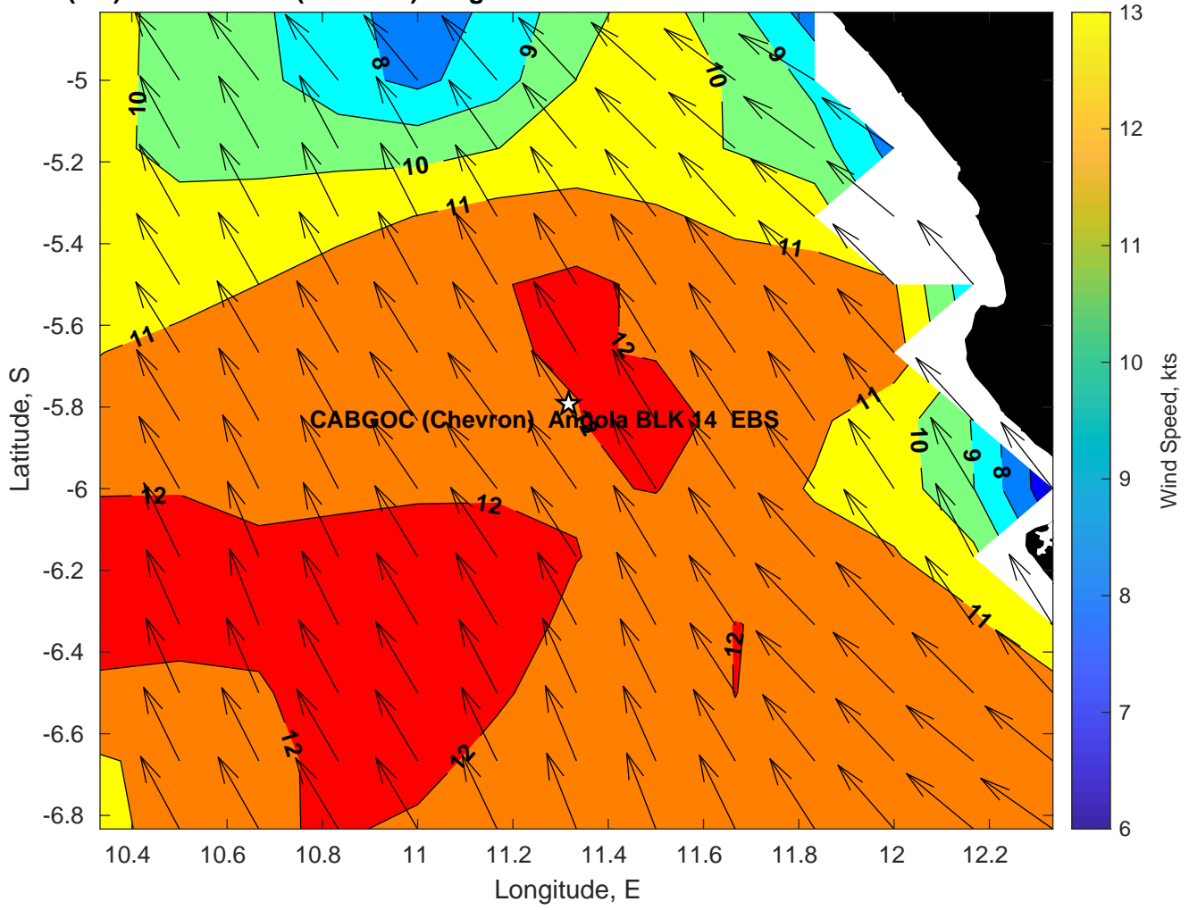
Winds (kts) for CABGOC (Chevron) Angola BLK 14 EBS at 30-Mar-2025 09:00:00
