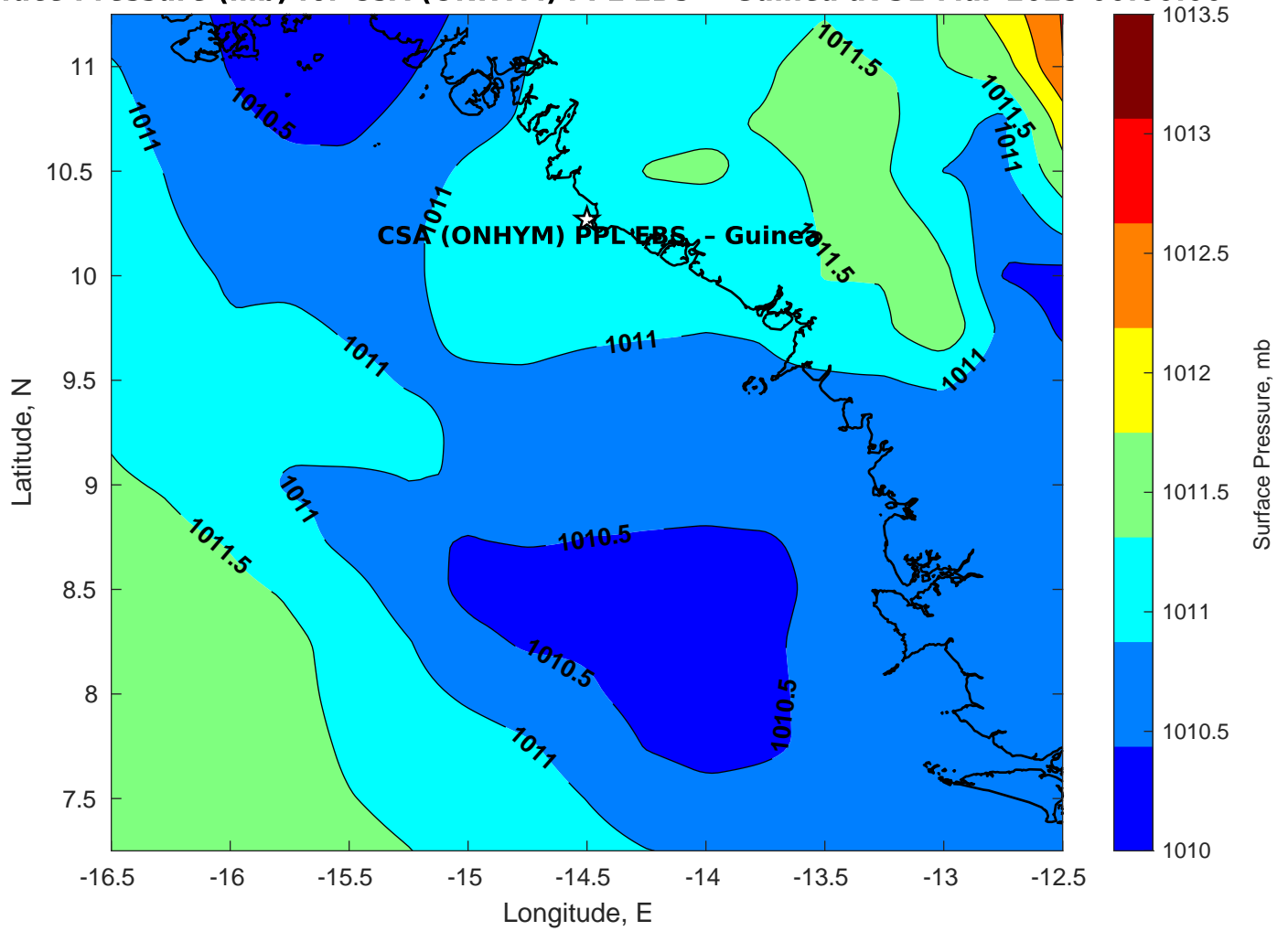
Surface Pressure (mb) for CSA (ONHYM) PPL EBS - Guinea at 31-Mar-2025 00:00:00
