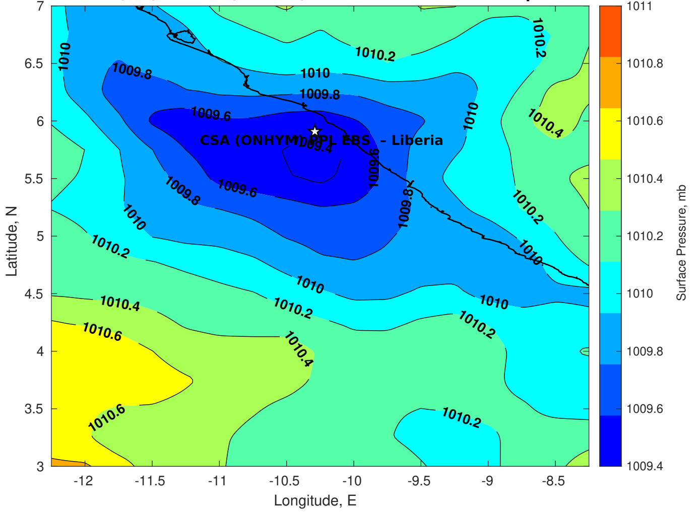
Surface Pressure (mb) for CSA (ONHYM) PPL EBS - Liberia at 01-Apr-2025 00:00:00
