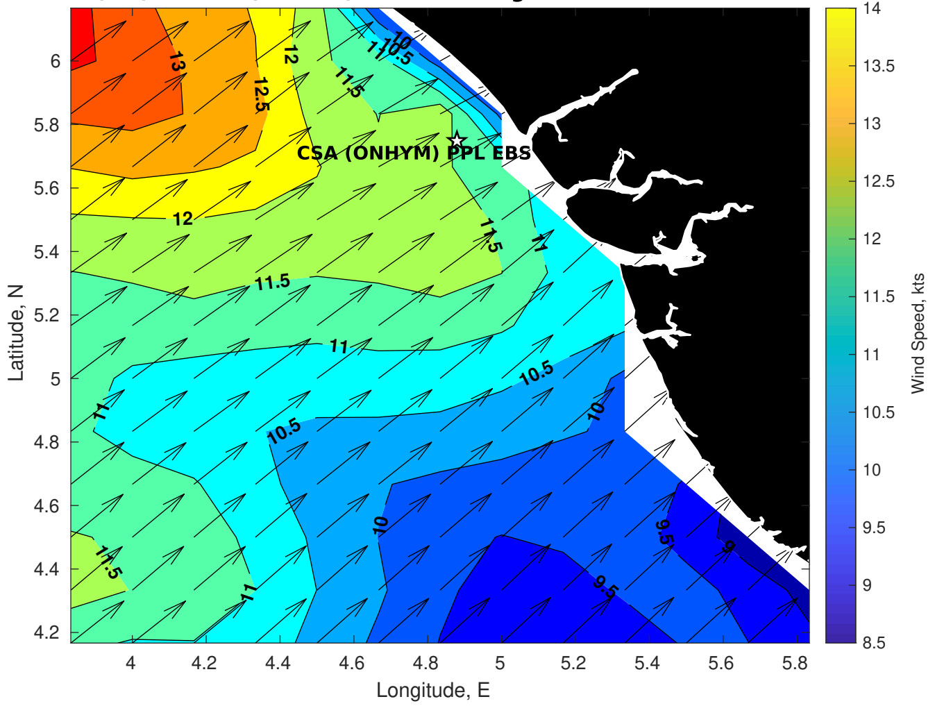
Winds (kts) for CSA (ONHYM) PPL EBS - Nigeria at 30-Mar-2025 09:00:00
