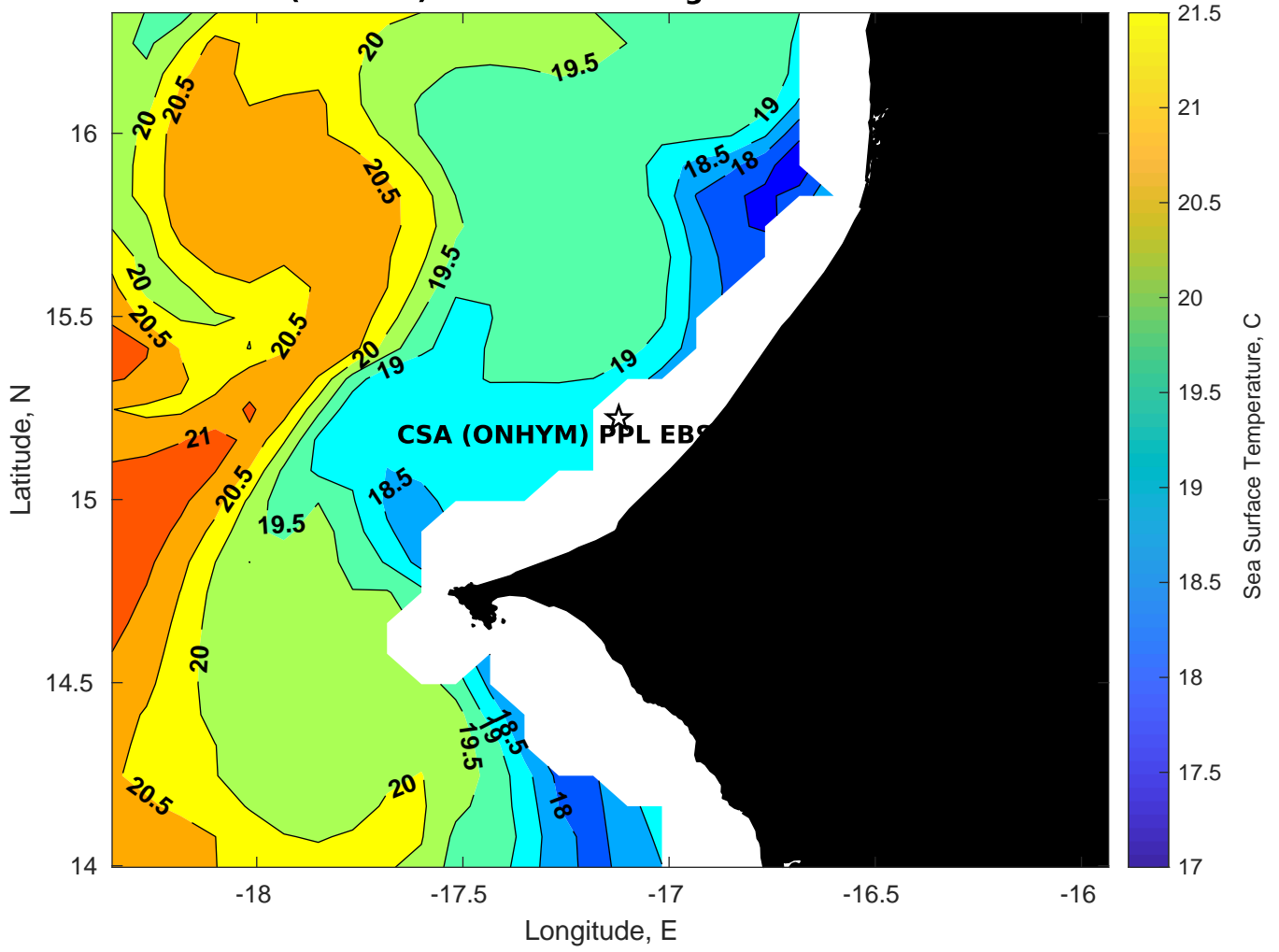
SST for CSA (ONHYM) PPL EBS - Senegal at 29-Mar-2025 00:00:00
