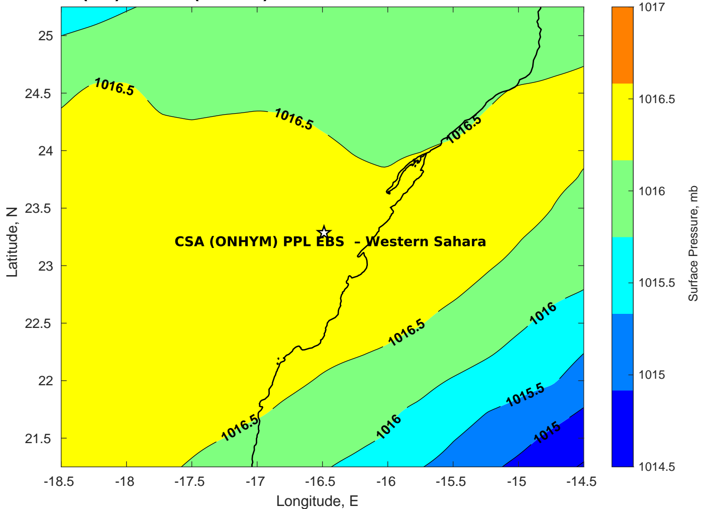
Surface Pressure (mb) for CSA (ONHYM) PPL EBS - Western Sahara at 31-Mar-2025 00:00:00
