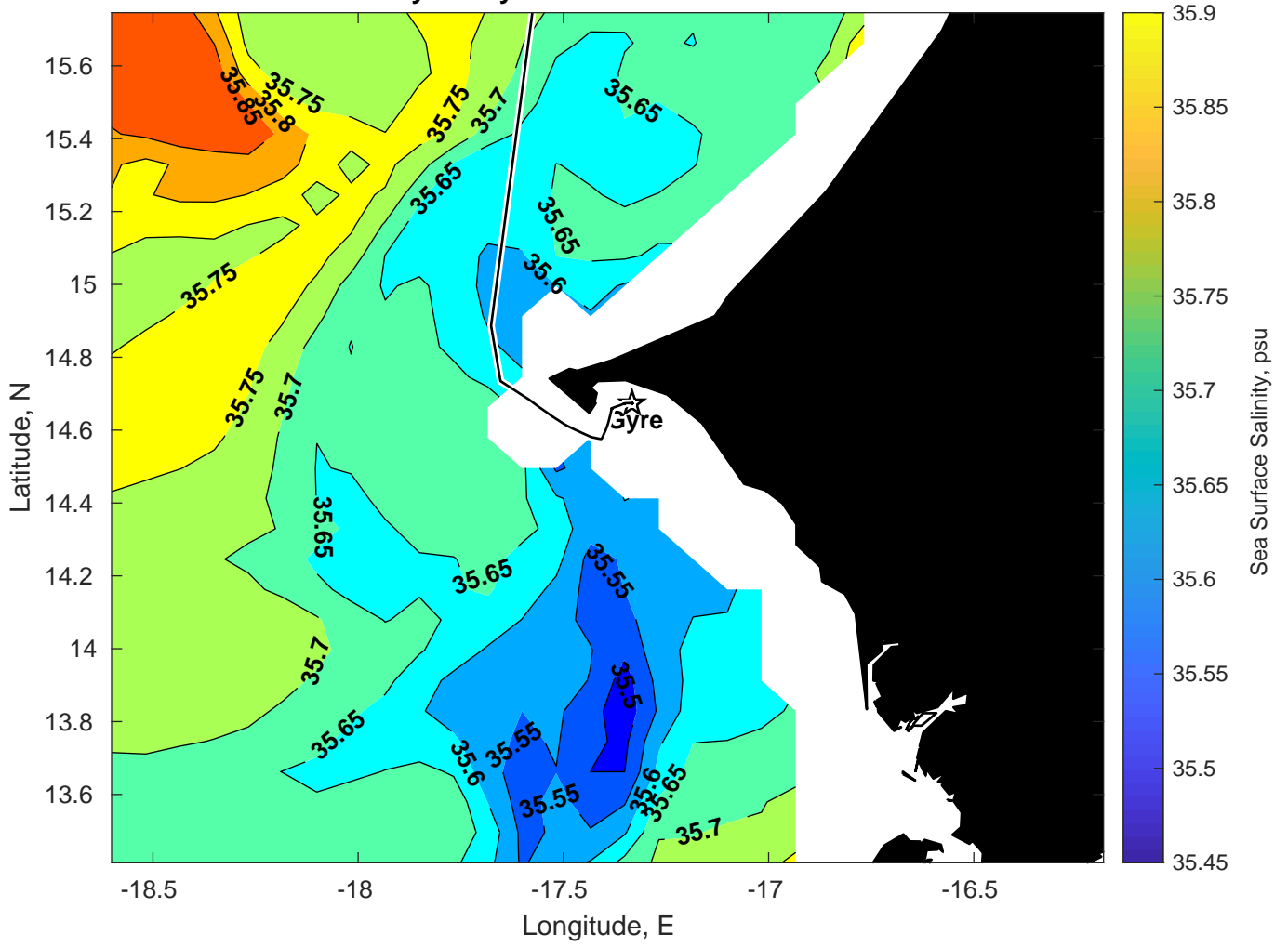
Surface Salinity for Gyre at 29-Mar-2025 00:00:00
