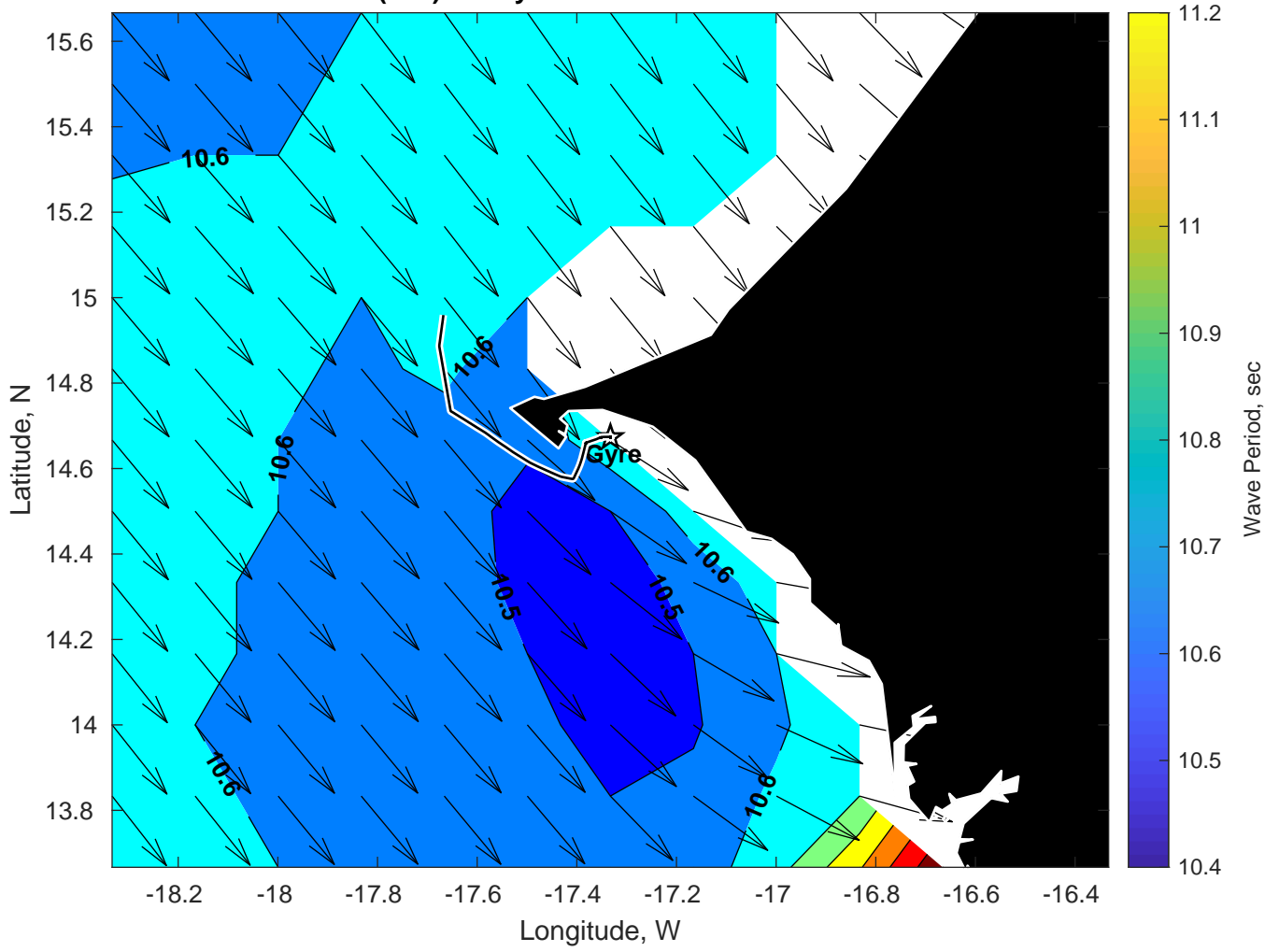
Wave Period (sec) for Gyre at 30-Mar-2025 09:00:00
