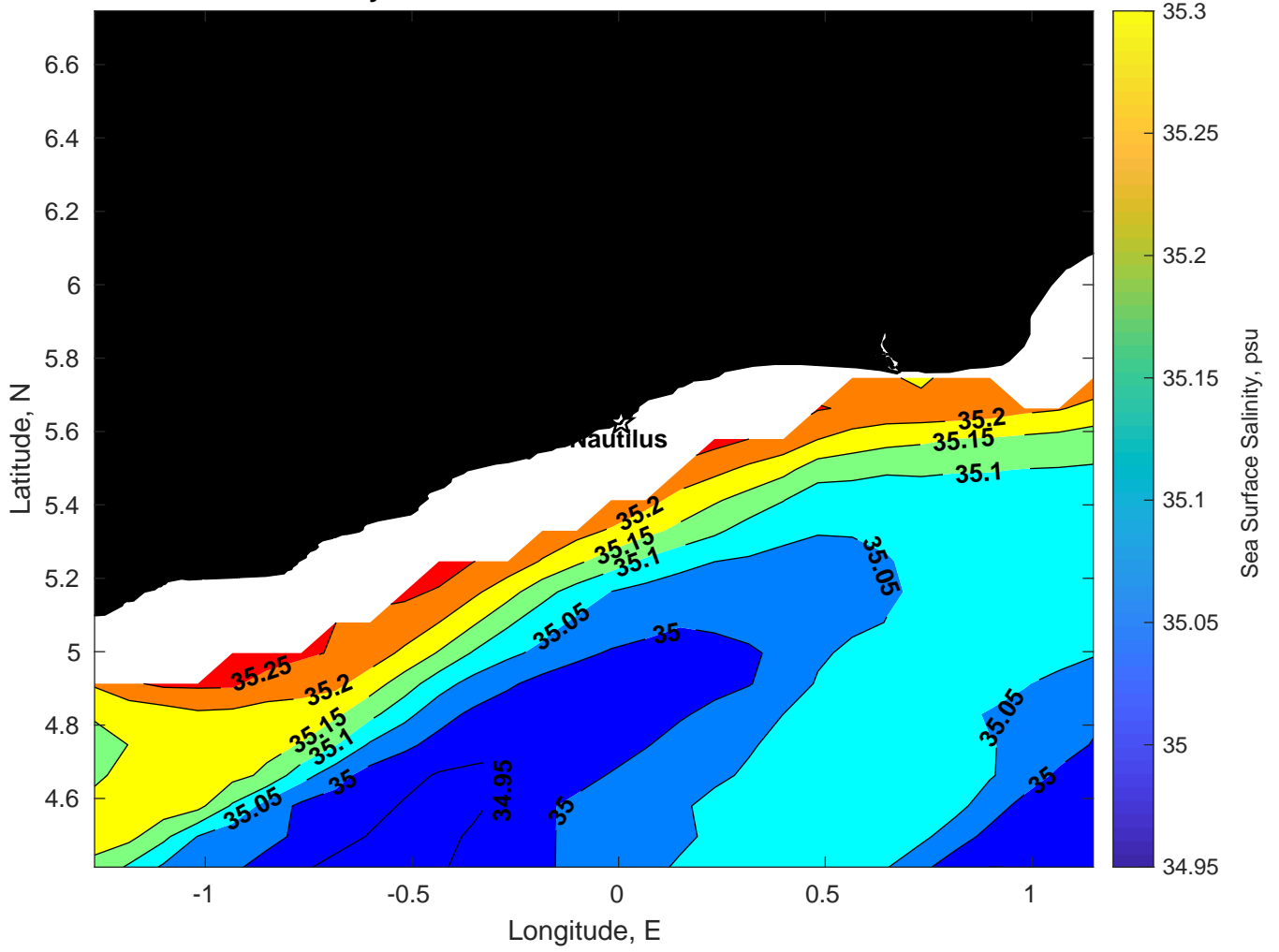
Surface Salinity for Nautilus at 29-Mar-2025 00:00:00
