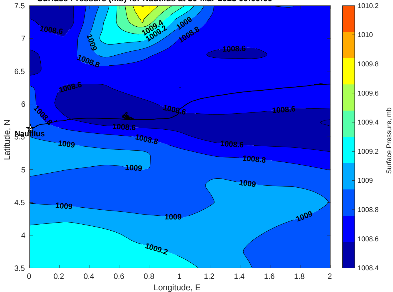
Surface Pressure (mb) for Nautilus at 30-Mar-2025 00:00:00
