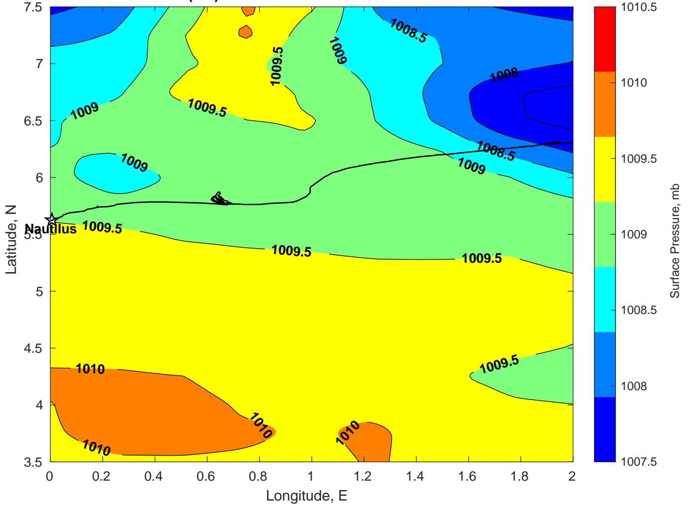
Surface Pressure (mb) for Nautilus at 31-Mar-2025 00:00:00
