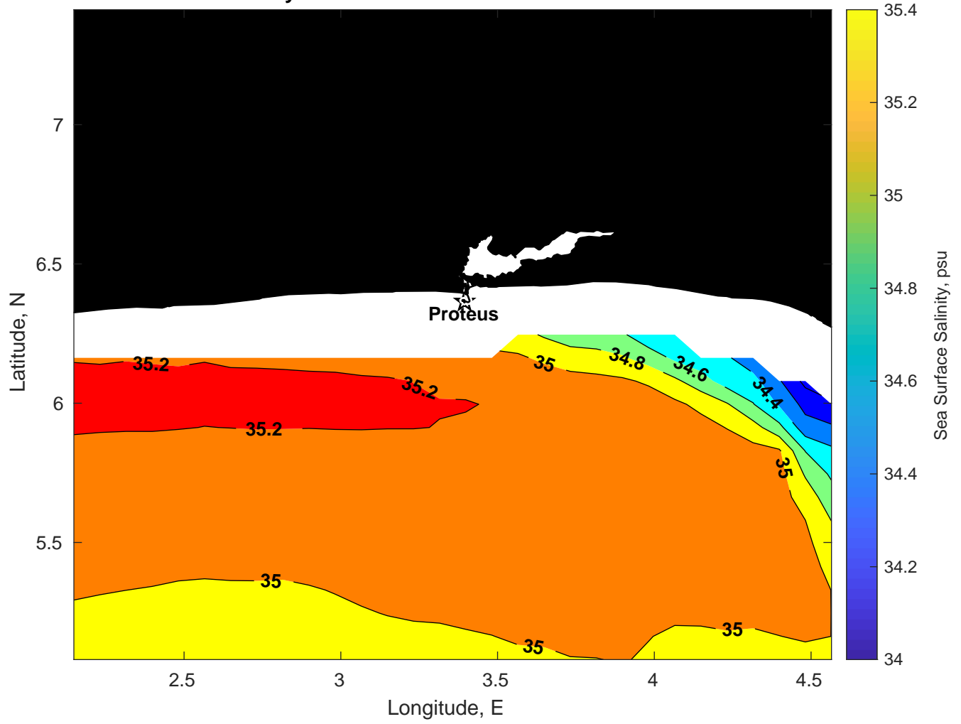
Surface Salinity for Proteus at 29-Mar-2025 00:00:00
