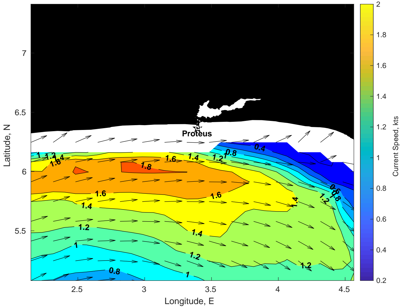
Surface Currents for Proteus at 29-Mar-2025 00:00:00
