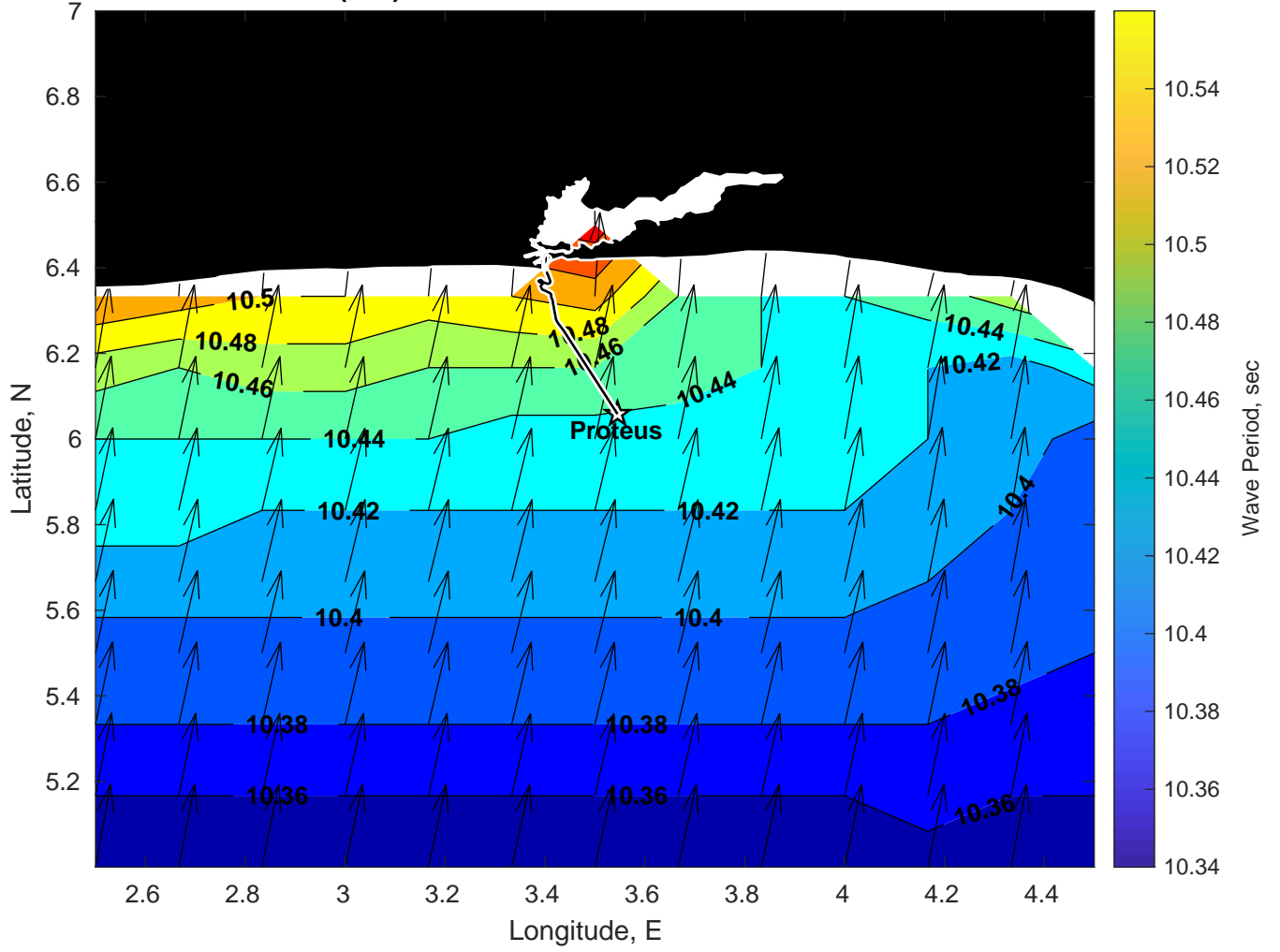
Wave Period (sec) for Proteus at 30-Mar-2025 09:00:00
