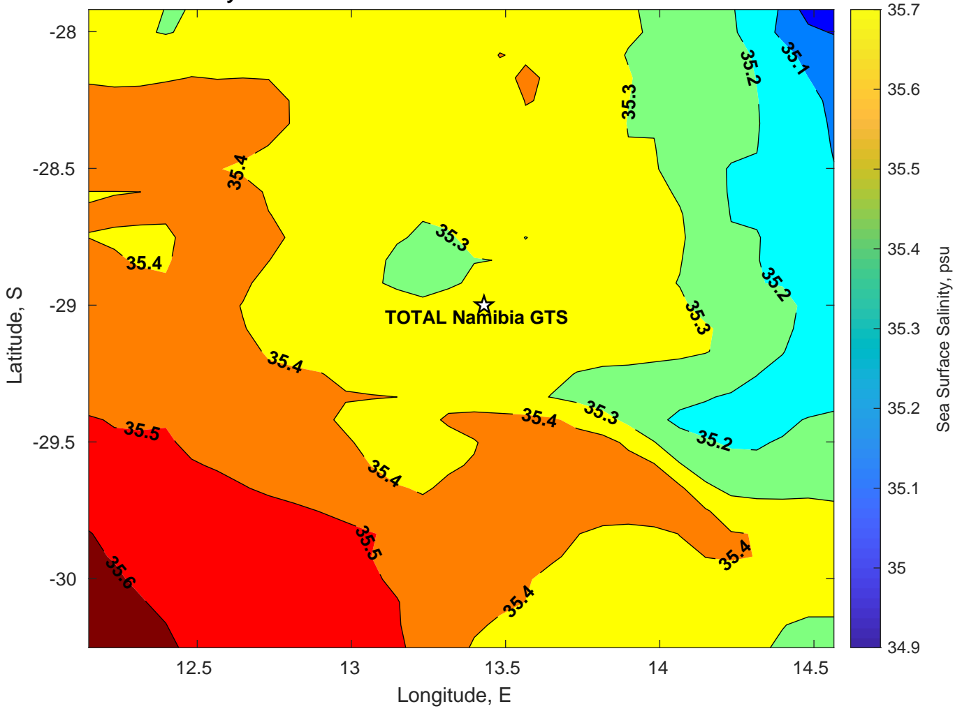
Surface Salinity for TOTAL Namibia GTS at 29-Mar-2025 00:00:00
