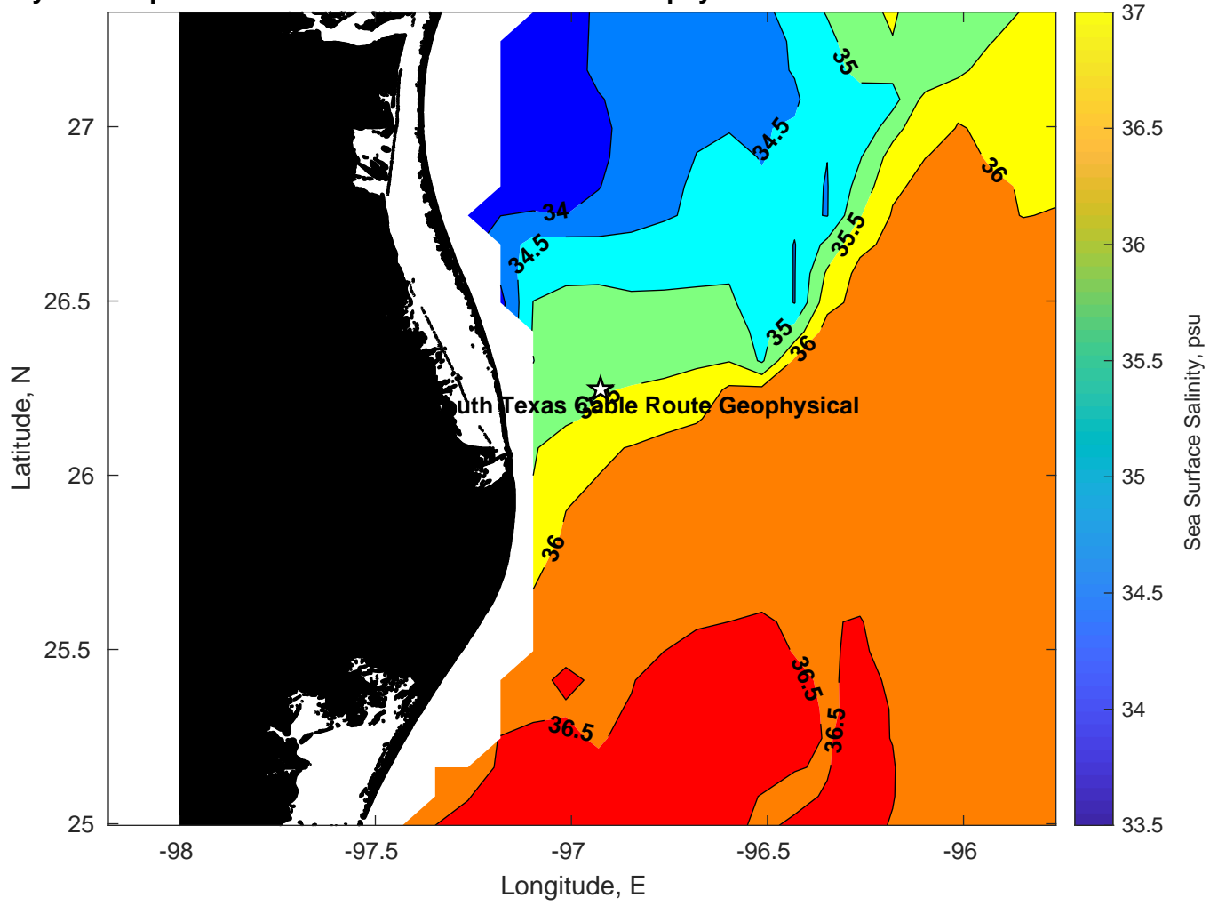
Surface Salinity for Tampnet P2378 South Texas Cable Route Geophysical at 29-Mar-2025 00:00:00
