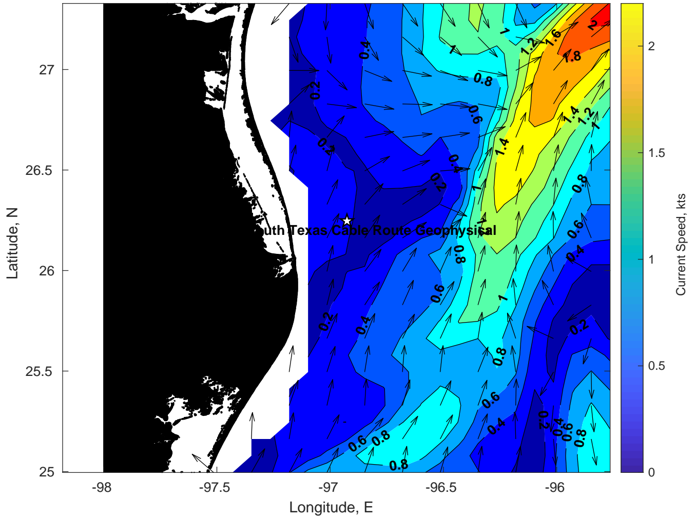
Surface Currents for Tampnet P2378 South Texas Cable Route Geophysical at 29-Mar-2025 00:00:00
