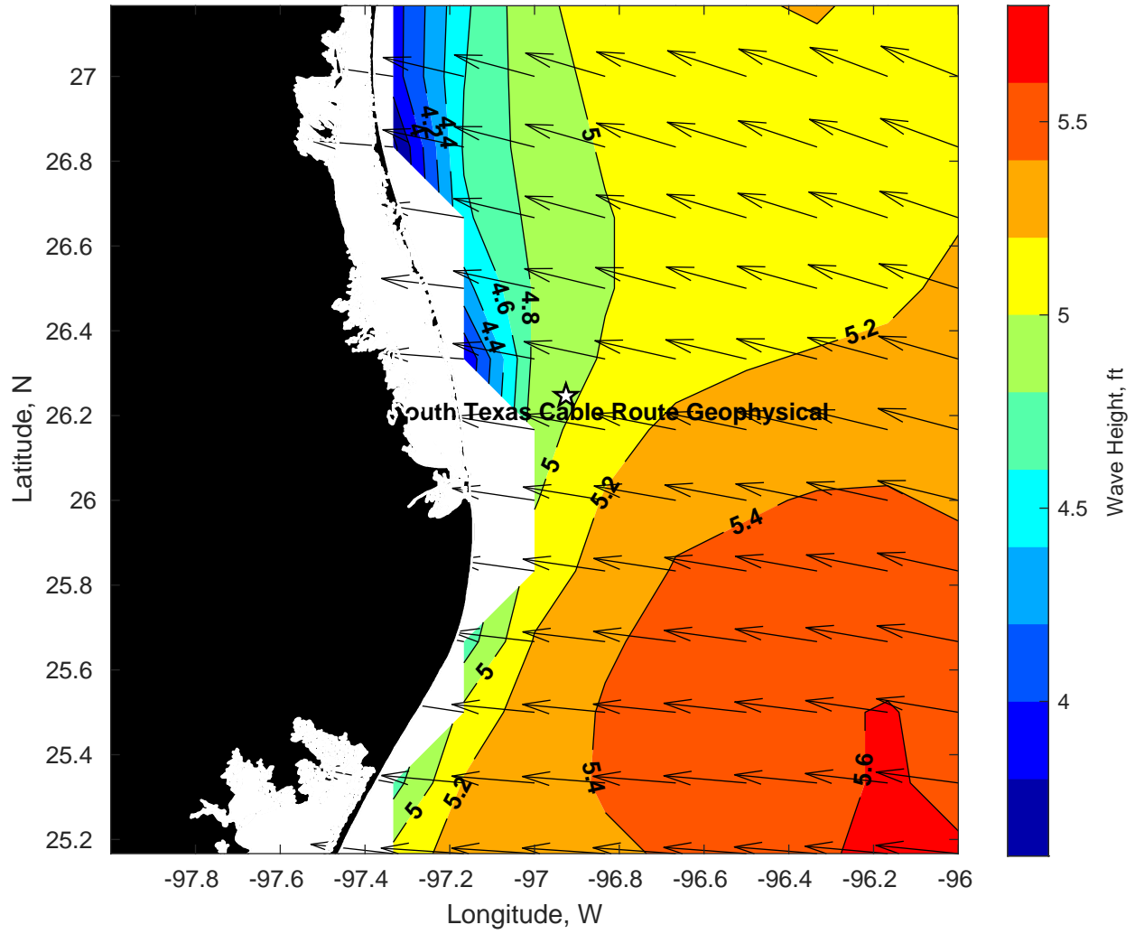
Wave Height (ft) for Tampnet P2378 South Texas Cable Route Geophysical at 30-Mar-2025 09:00:00
