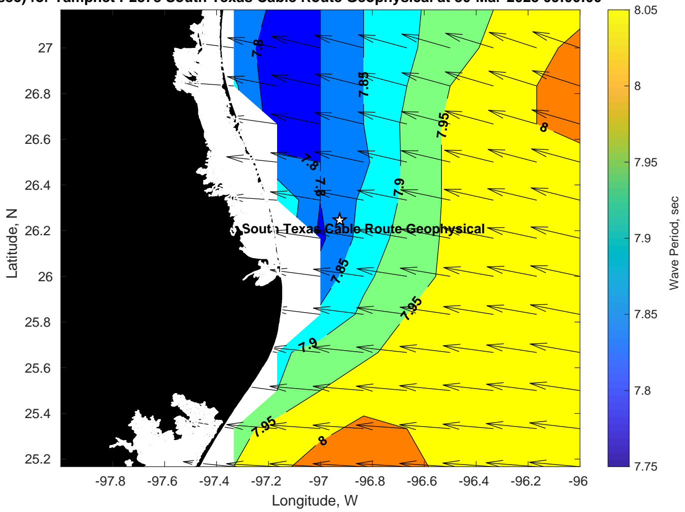
Period (sec) for Tampnet P2378 South Texas Cable Route Geophysical at 30-Mar-2025 09:00:00
