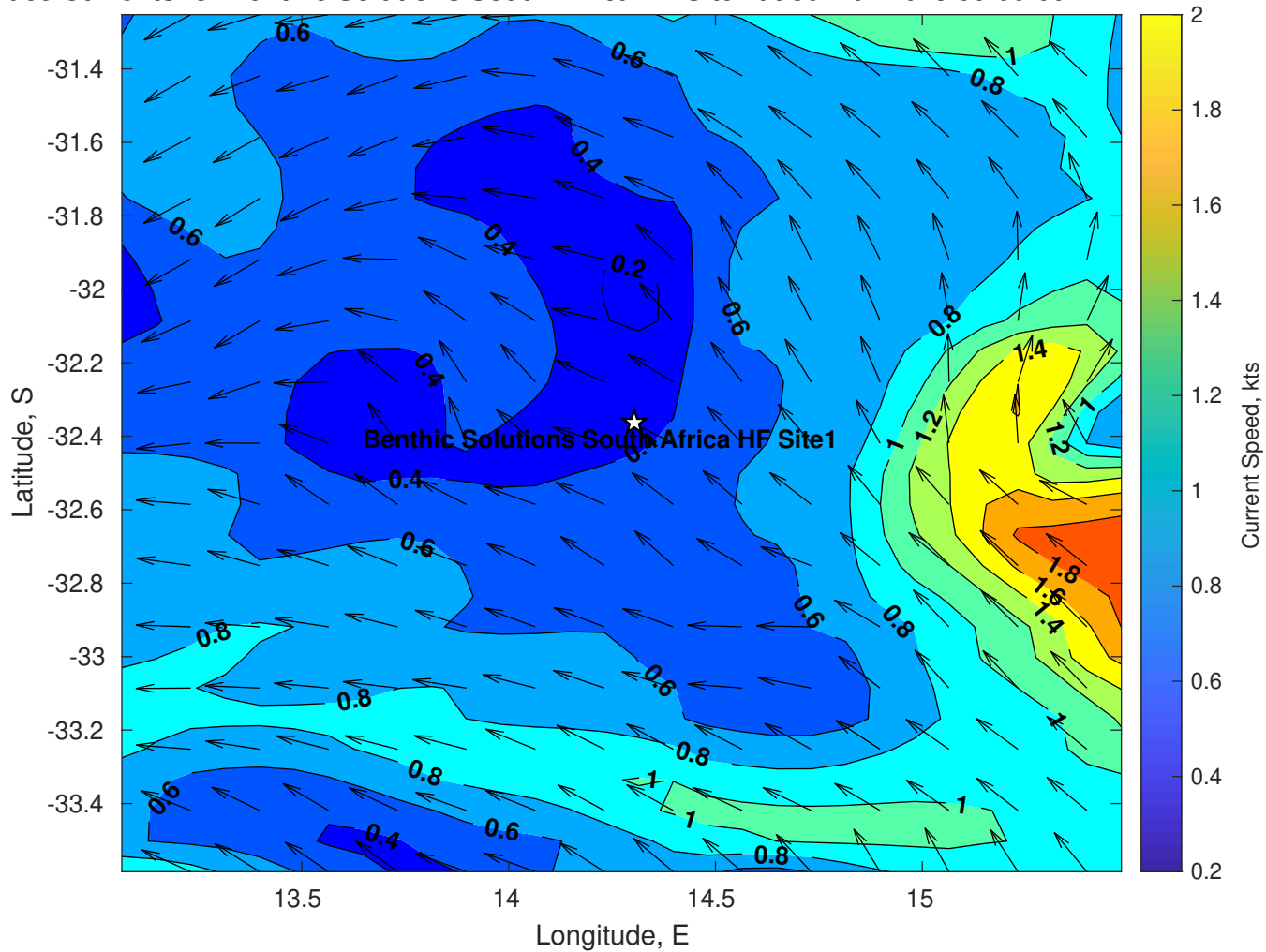
Surface Currents for Benthic Solutions South Africa HF Site1 at 30-Mar-2025 00:00:00
