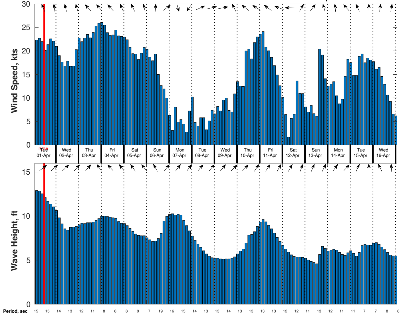
Wind & Wave Forecast for Benthic Solutions South Africa HF Site1 from 31-Mar-2025 02:00:00 to 16-Apr-2025 02:00:00
