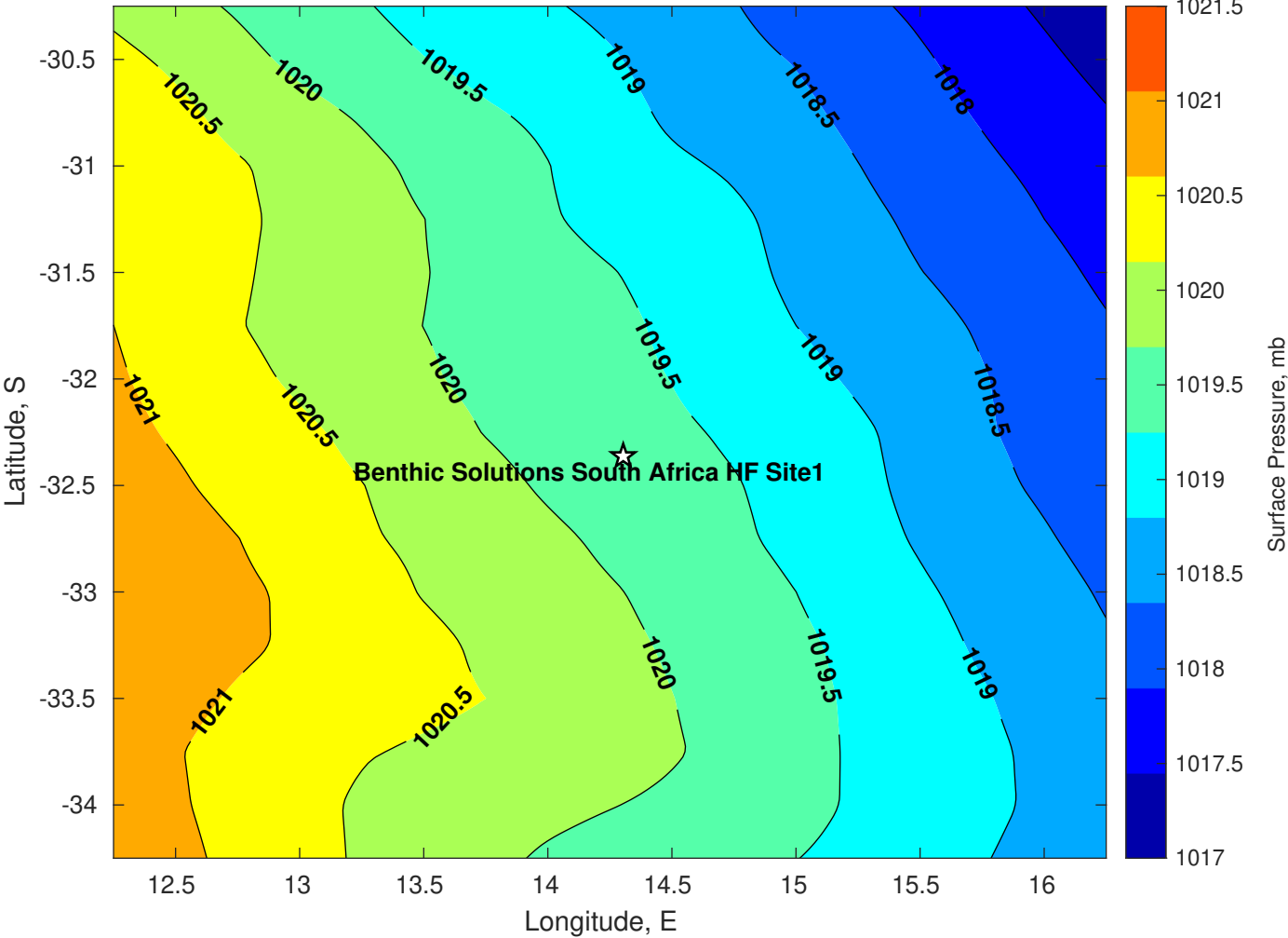
Surface Pressure (mb) for Benthic Solutions South Africa HF Site1 at 01-Apr-2025 00:00:00
