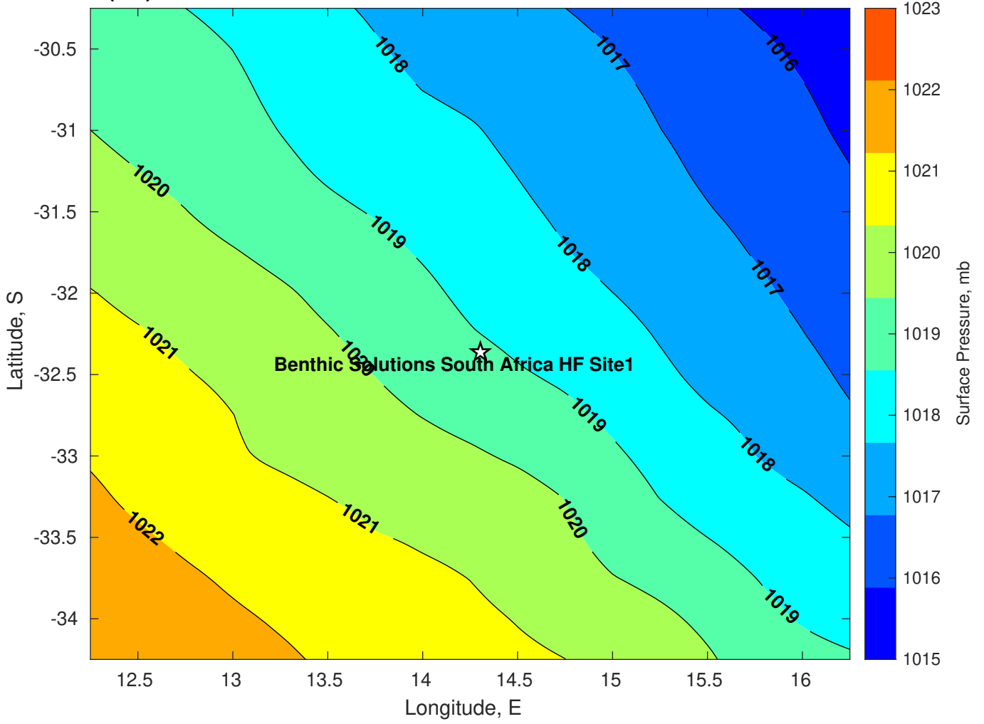
Surface Pressure (mb) for Benthic Solutions South Africa HF Site1 at 31-Mar-2025 00:00:00
