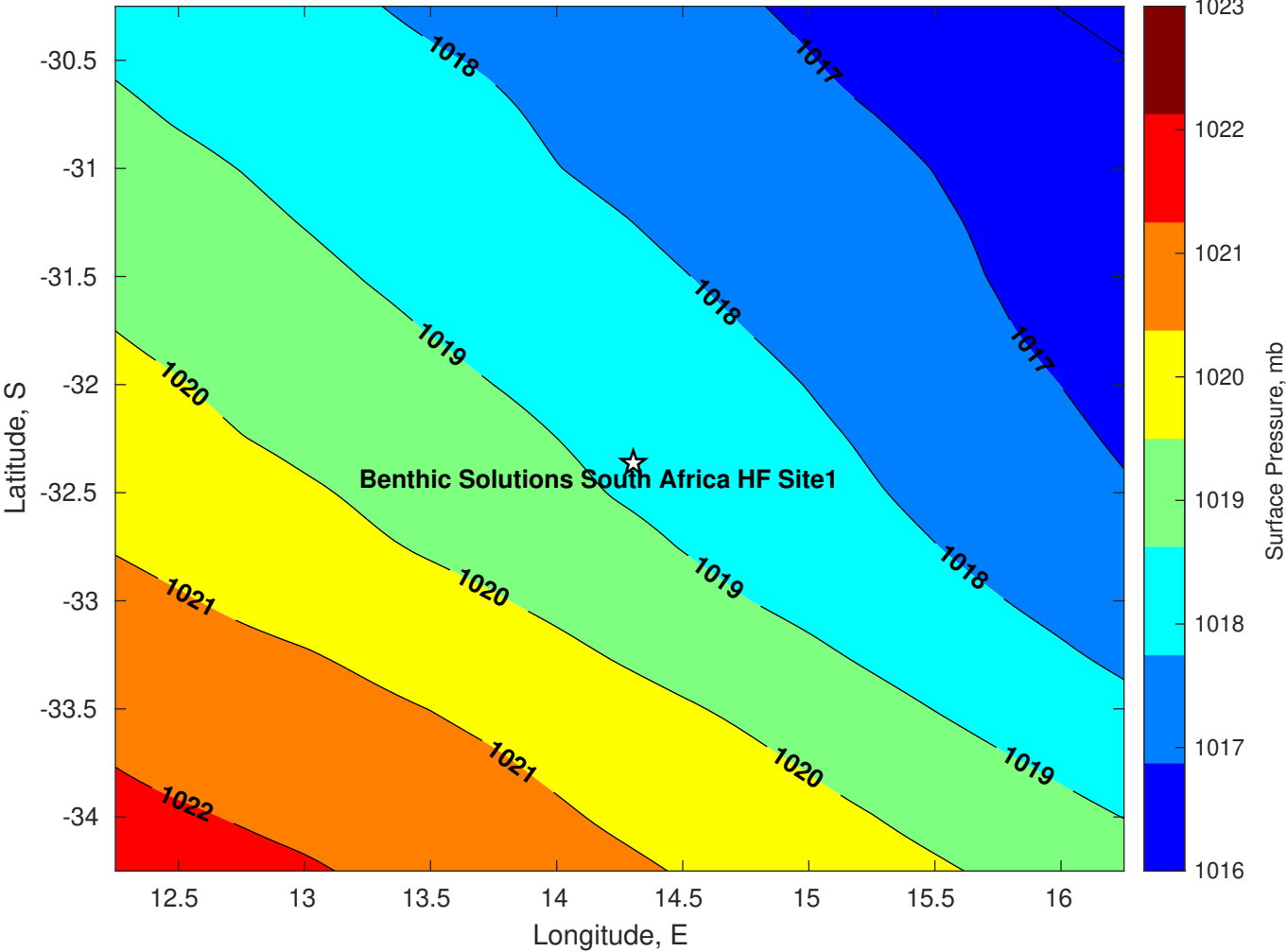
Surface Pressure (mb) for Benthic Solutions South Africa HF Site1 at 02-Apr-2025 00:00:00
