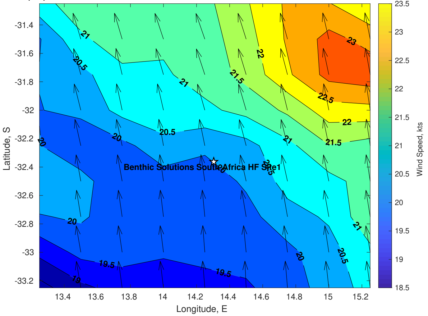
Winds (kts) for Benthic Solutions South Africa HF Site1 at 31-Mar-2025 09:00:00
