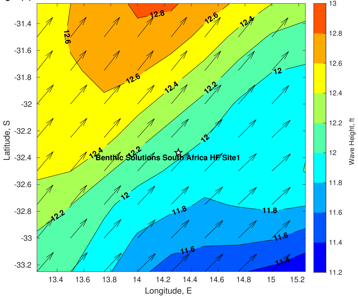
Wave Height (ft) for Benthic Solutions South Africa HF Site1 at 31-Mar-2025 09:00:00
