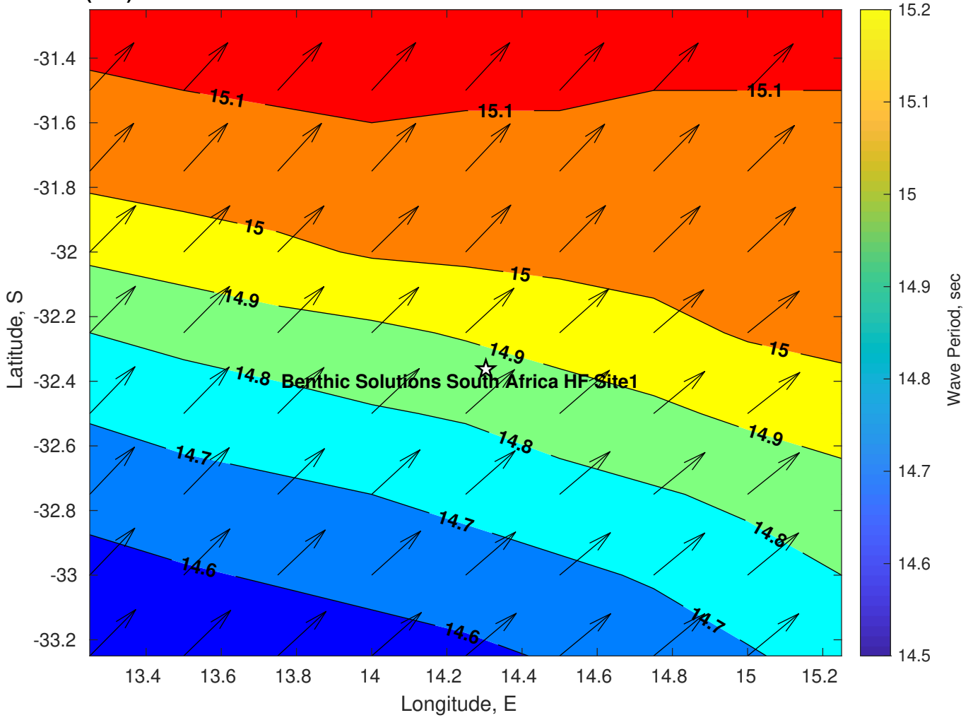
Wave Period (sec) for Benthic Solutions South Africa HF Site1 at 31-Mar-2025 09:00:00
