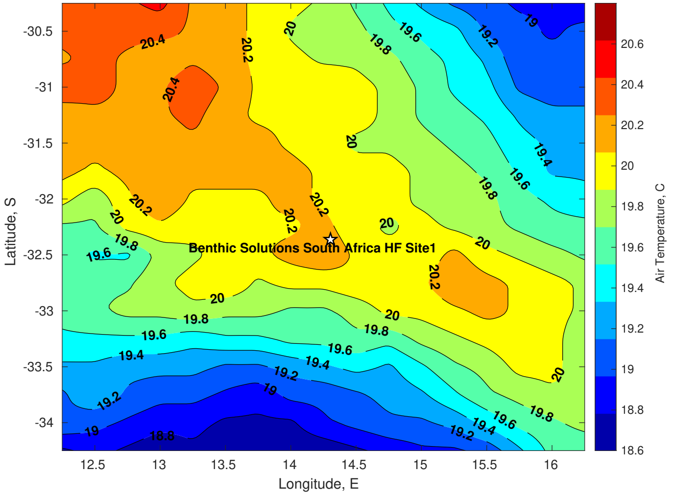
Air Temperature (C) for Benthic Solutions South Africa HF Site1 at 31-Mar-2025
