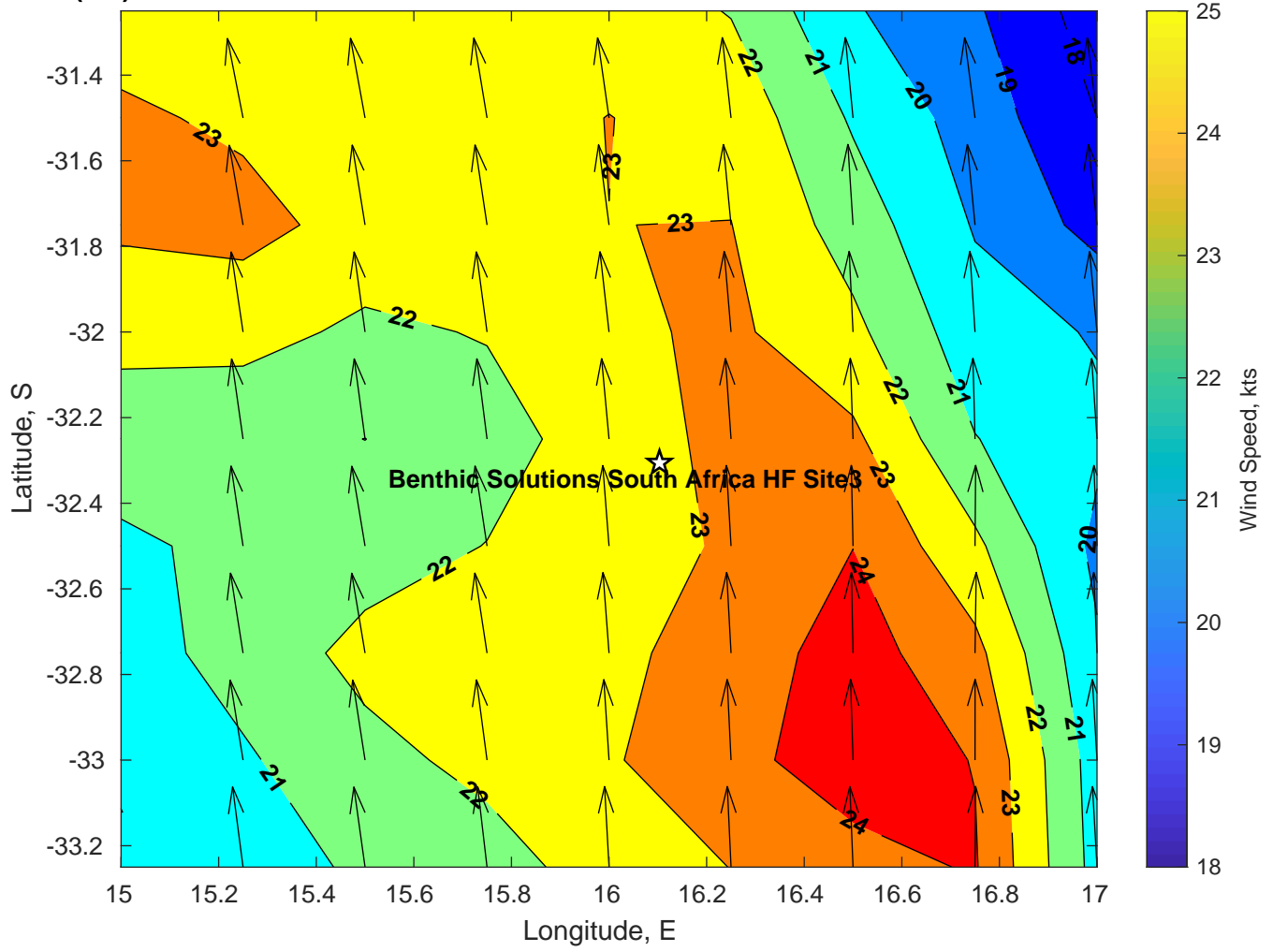
Winds (kts) for Benthic Solutions South Africa HF Site3 at 31-Mar-2025 09:00:00
