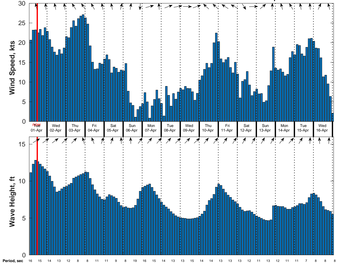
Wind & Wave Forecast for Benthic Solutions South Africa HF Site3 from 31-Mar-2025 02:00:00 to 16-Apr-2025 02:00:00
