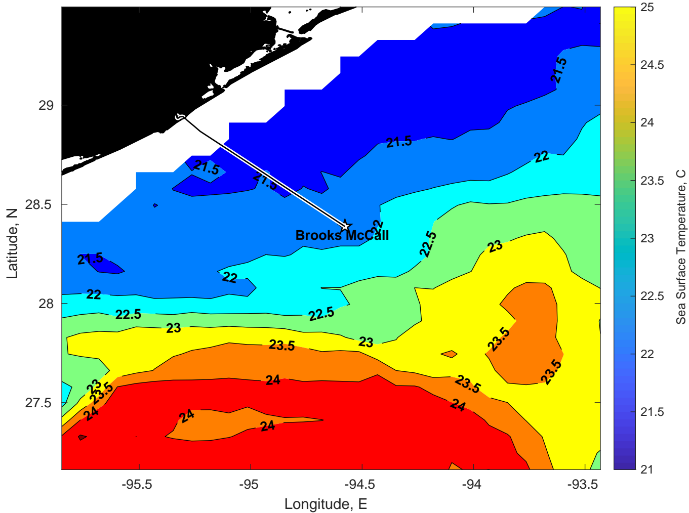
SST for Brooks McCall at 30-Mar-2025 00:00:00
