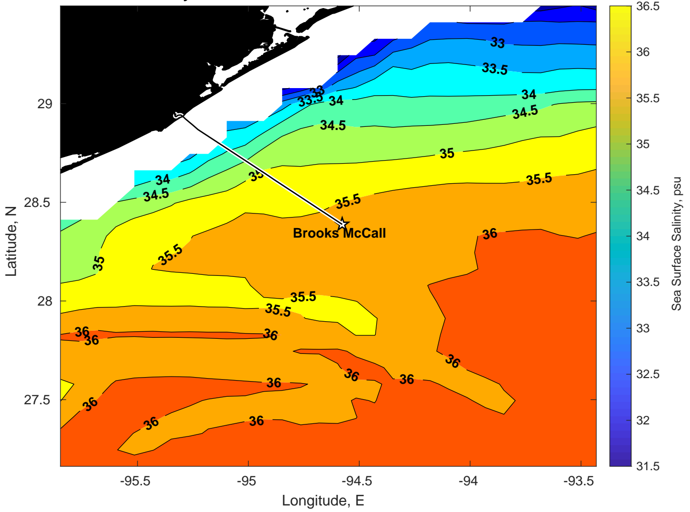
Surface Salinity for Brooks McCall at 30-Mar-2025 00:00:00
