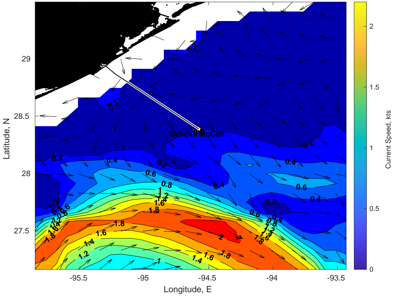
Surface Currents for Brooks McCall at 30-Mar-2025 00:00:00
