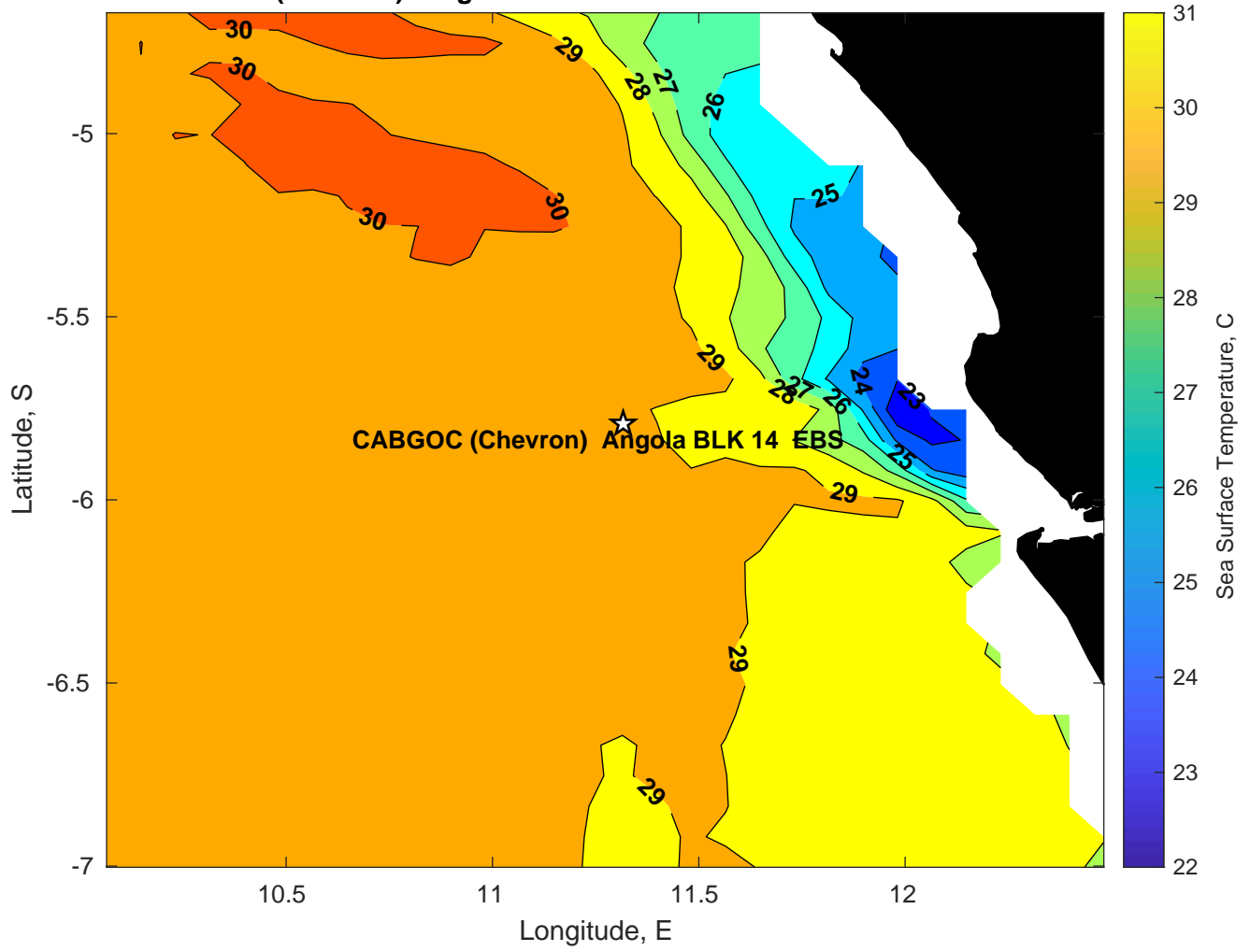
SST for CABGOC (Chevron) Angola BLK 14 EBS at 30-Mar-2025 00:00:00
