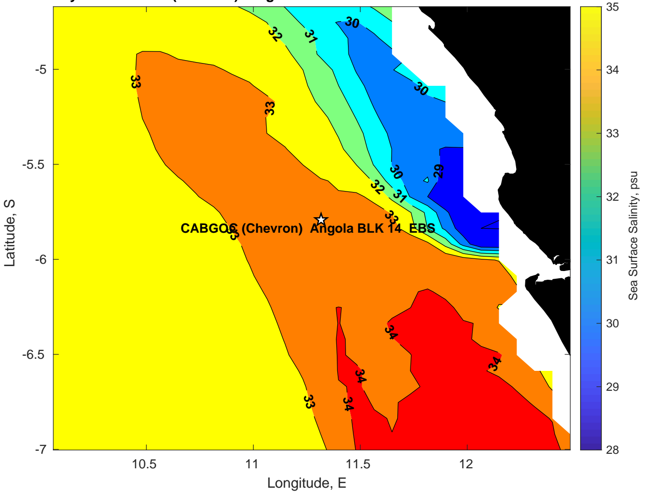
Surface Salinity for CABGOC (Chevron) Angola BLK 14 EBS at 30-Mar-2025 00:00:00
