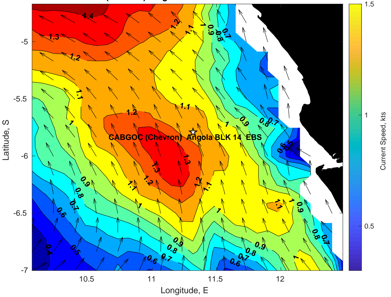
Surface Currents for CABGOC (Chevron) Angola BLK 14 EBS at 30-Mar-2025 00:00:00
