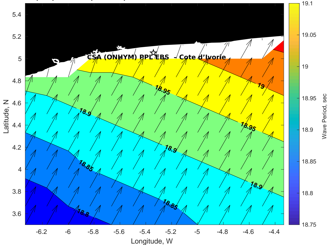
Wave Period (sec) for CSA (ONHYM) PPL EBS - Cote d'Ivoire at 31-Mar-2025 09:00:00
