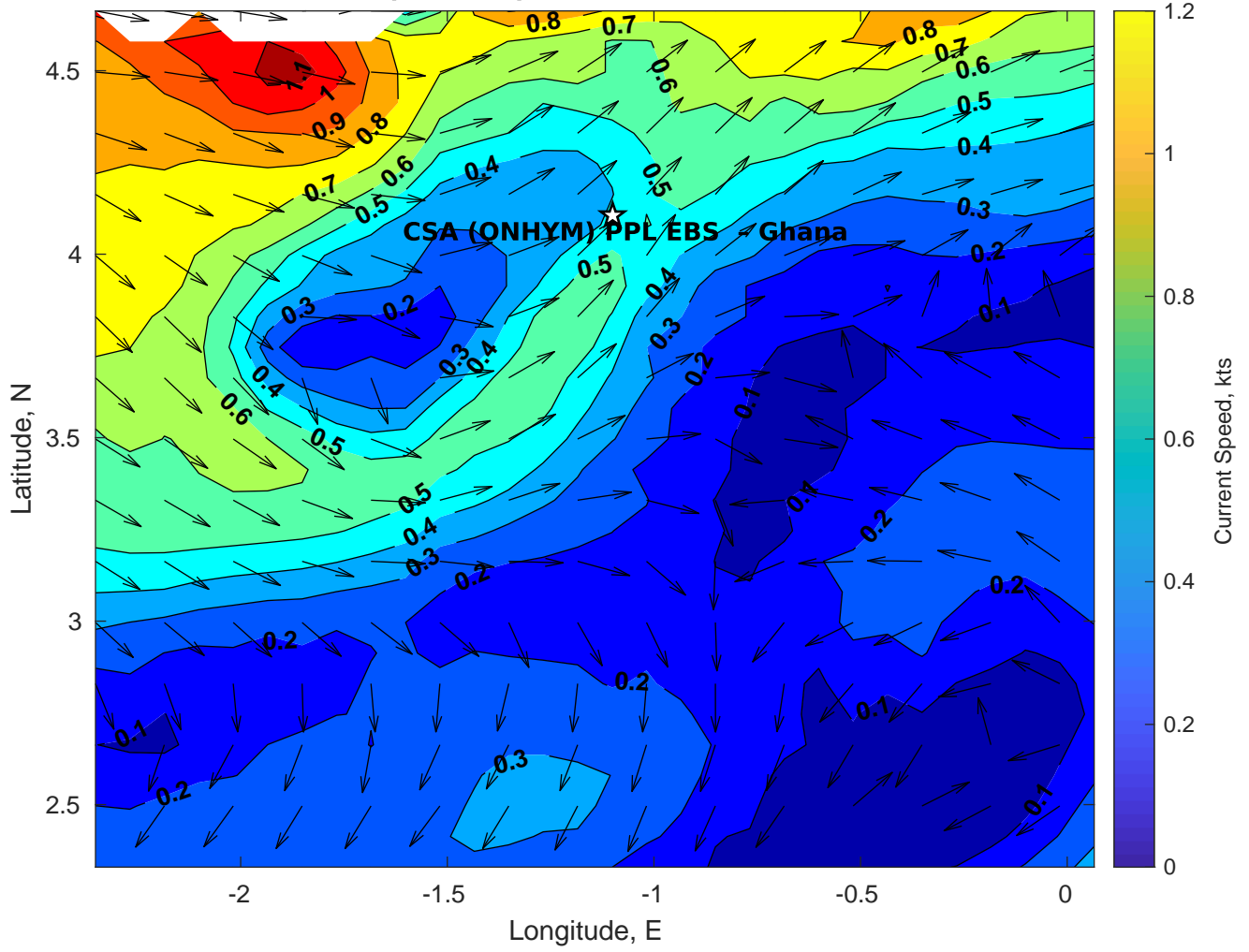
Surface Currents for CSA (ONHYM) PPL EBS - Ghana at 30-Mar-2025 00:00:00
